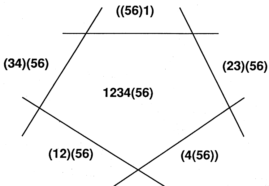
Figure 5. Boundary of 1234(56)
