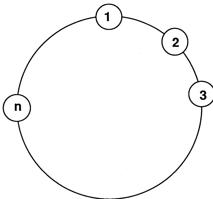
Figure 1. Juzu 12...n
