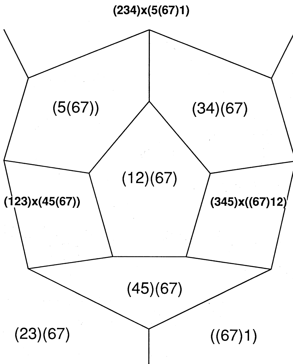
Figure 8. Boundary of 12345(67)
