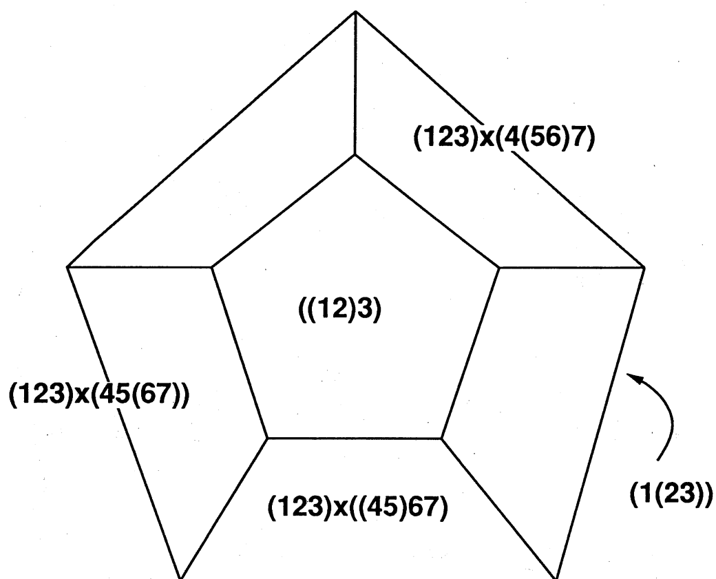
Figure 9. Prism (123)x(4567)
