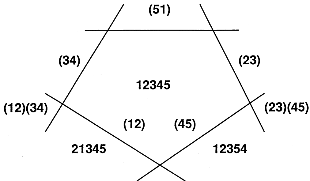
Figure 3. Boundary of 12345
