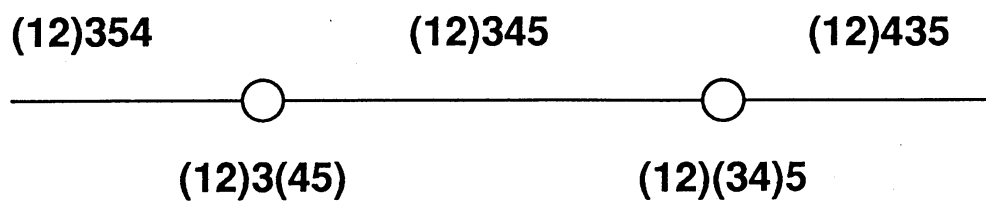
Figure 2. Segment (12)345
