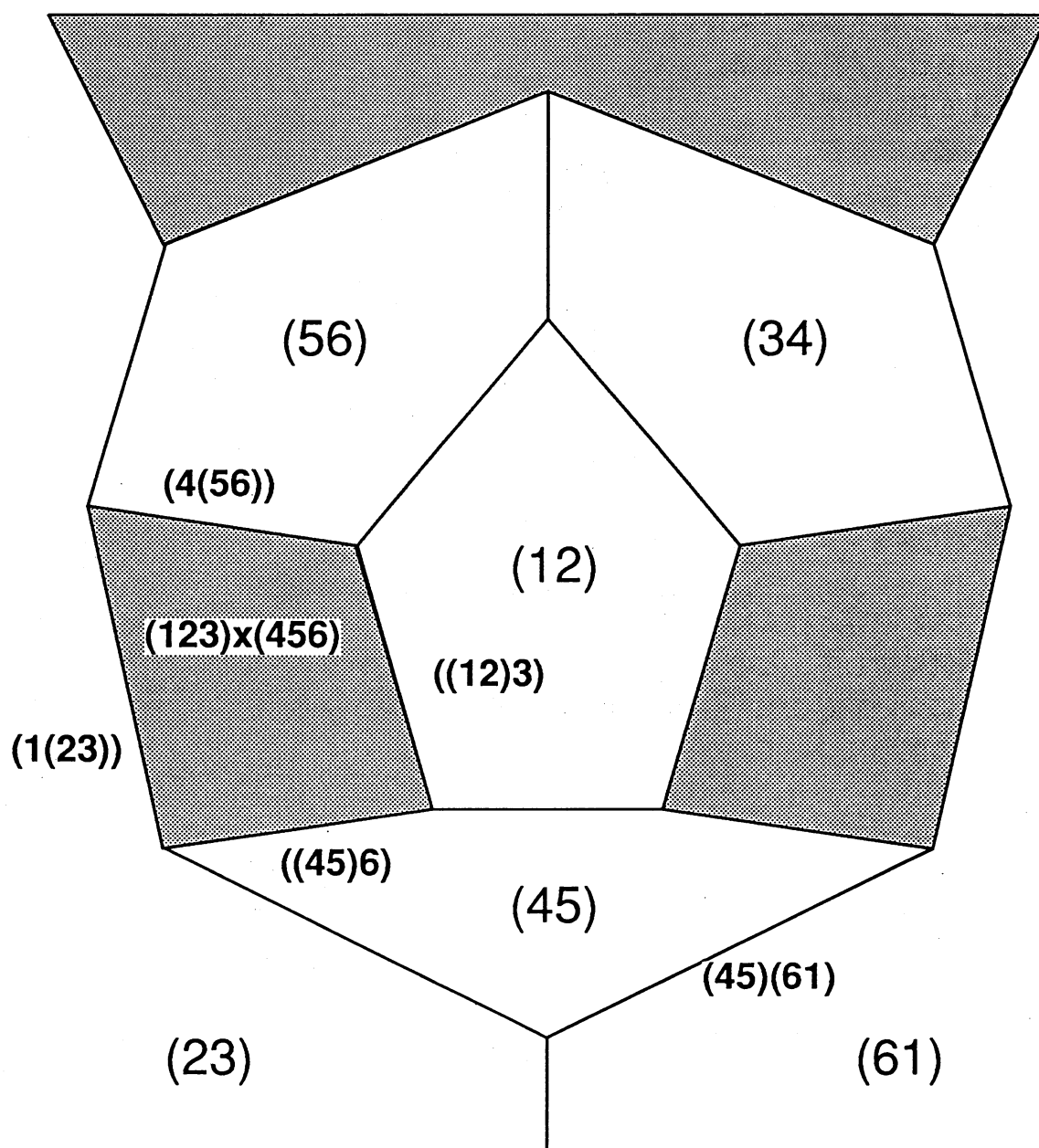
Figure 6. Boundary of 123456
