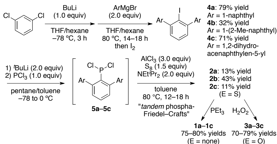
Scheme 2. Synthesis of 1–3
