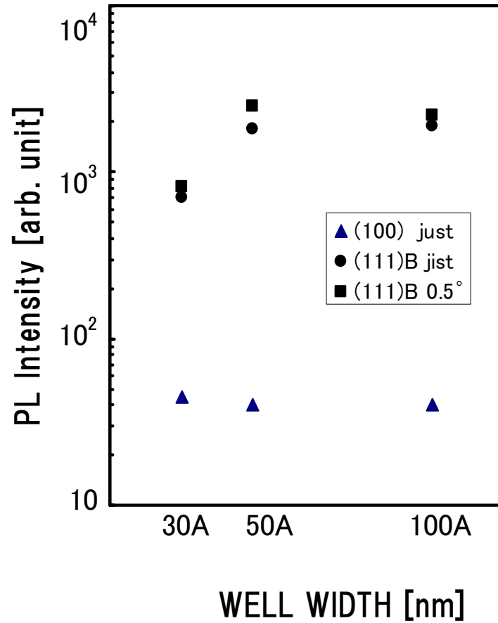
Fig. 1.23 Photoluminescence intensity of AlGaAs-GaAs SQWs grown on (100) , exact (111)\text{B} and mis-oriented (111)\text{B} substrates.
