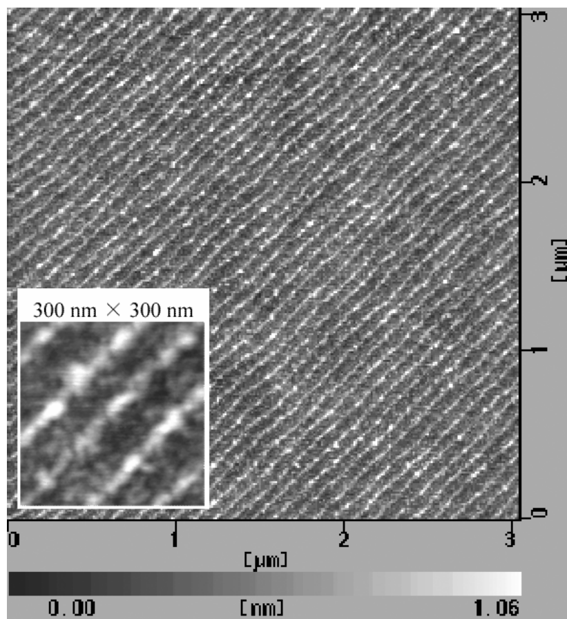
Fig. 2.2 AFM images of dot alignment along steps on sapphire substrates. The condition of the formation was at 700^{\circ}\text{C} for 10 seconds by MOCVD: (a) the large area image and (b) enlarged image of the surface.
