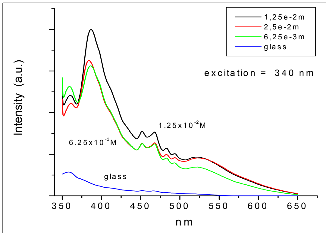
Fig. 2.6 Fluorescence spectra.
