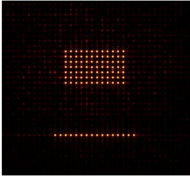
Fig. 3.7 Simulated typical light-intensity distribution used for parallel irradiation of 7 \times 12 spots.
