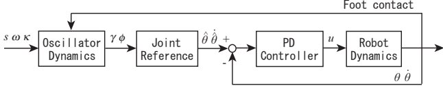
Fig. 2 Block diagram of the control system
