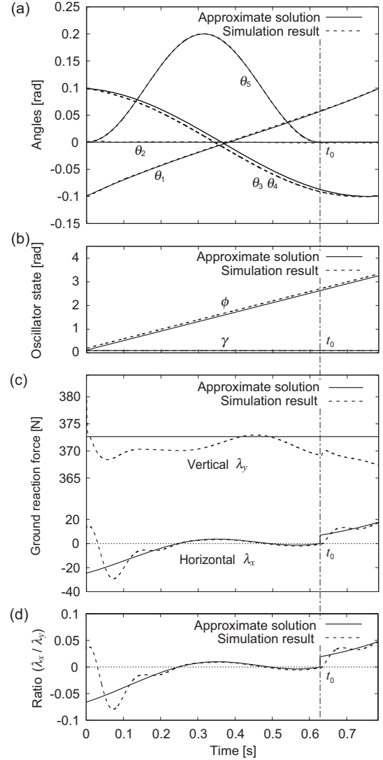
Fig. 5 Comparison between approximate solutions and simulation results. (a) Angles, (b) oscillator states, and (c) ground reaction forces. (d) Ratio between horizontal and vertical reaction forces.
