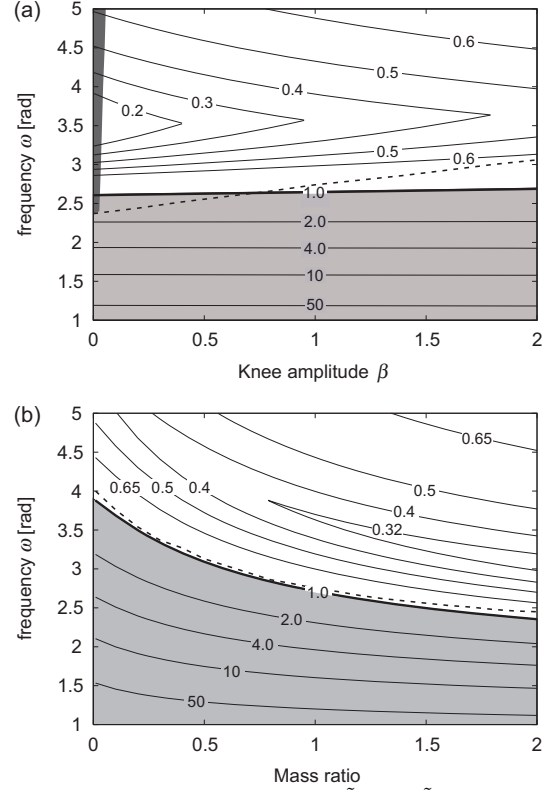
Fig. 7 Maximum eigenvalue between \tilde{\Lambda}_3 and \tilde{\Lambda}_4 . The light gray area indicates the unstable region, and dark gray area indicates the area in which the swing leg scrapes during walking. The bold and dotted lines indicate the stability boundaries of the approximate analysis and the rigorous simulation results, respectively. (a) Knee amplitude and locomotion speed. (b) Mass ratio of the torso and locomotion speed.
