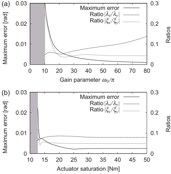
Fig. 4 Effects of gain parameters in (a) joint feedback control and (b) actuator saturation, showing the maximum error among joint errors |\theta_i - \hat{\theta}_i| ( i = 2, \dots, 5 ) and ratios between horizontal and vertical reaction forces |\lambda_x/\lambda_y| and between horizontal and vertical impulse at foot contact |\xi_x/\xi_y| . In the gray area, the walking model falls down.
