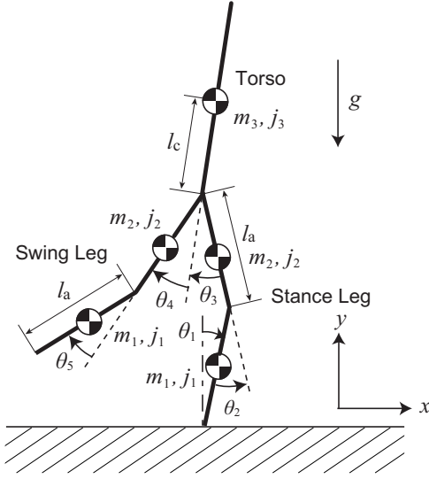
Fig. 1 Schematic diagram of the five-link planar biped robot
