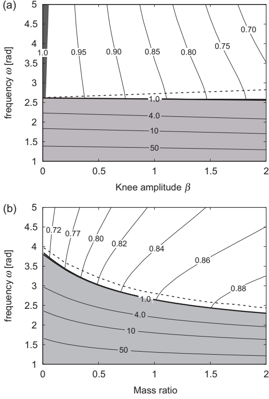
Fig. 6 Maximum eigenvalue between \Lambda_3 and \Lambda_4 . The light gray area is the unstable region, and, in the dark gray area, the swing leg scrapes during walking. The bold and dotted lines indicate the stability boundaries of the approximate analysis and rigorous simulation results, respectively. (a) Effects of knee motion and locomotion speed. (b) Effects of the mass ratio of the torso and the locomotion speed.
