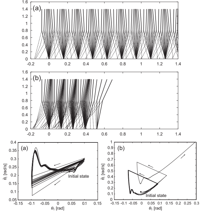
Fig. 3 Stick diagram of walking behavior and postural motion \theta_1 and \dot{\theta}_1 . (a) \omega = 4.0 rad. Walking motion converges to periodic motion. (b) \omega = 2.5 rad. The walking model falls forward, and the trajectory diverges from periodic behavior.
