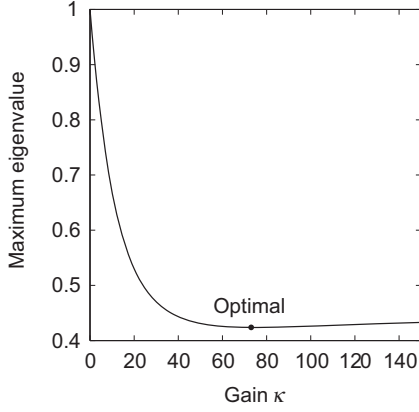
Fig. 8 Optimal value for gain parameter \kappa to minimize the maximum eigenvalue
