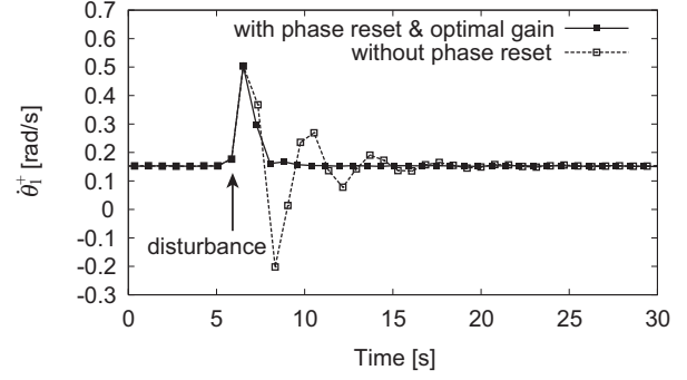
Fig. 9 Behavior of angular velocity \dot{\theta}_1^+ of the posture angle just after foot contact, for the case of the addition of a disturbance
