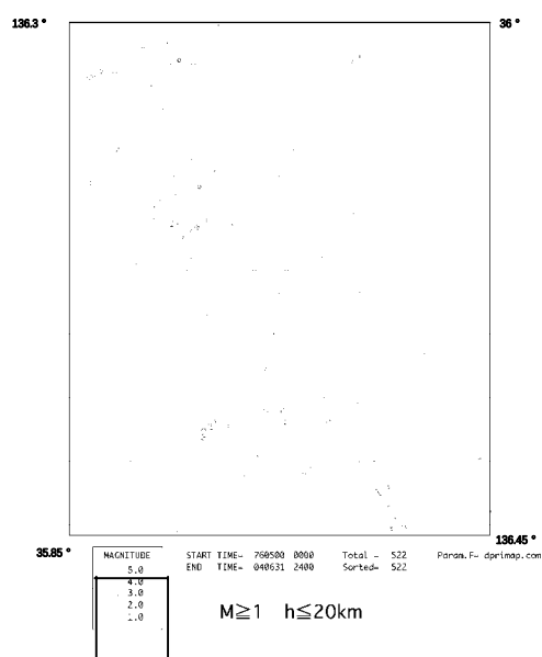
Fig.3 Seismicity of Ikeda town from 1976.05-2004.06.
