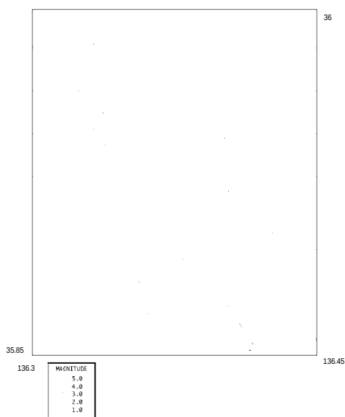
Fig.4 Seismic gap appeared before occurrence of main shock
