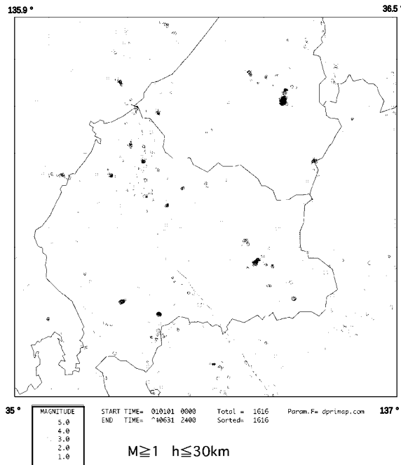
Fig.6 Seismicity of Reihoku district.
