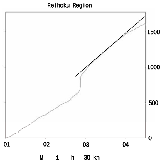
Fig.7 Cumulative number for Reihoku district.
