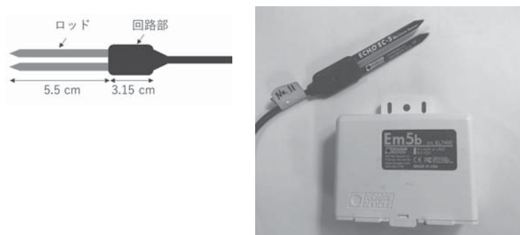
Fig. 1 Size of EC-5 Soil Moisture Sensor (Left), Picture of EC-5 Soil Moisture Sensor, Em5b Data Logger (Right)
