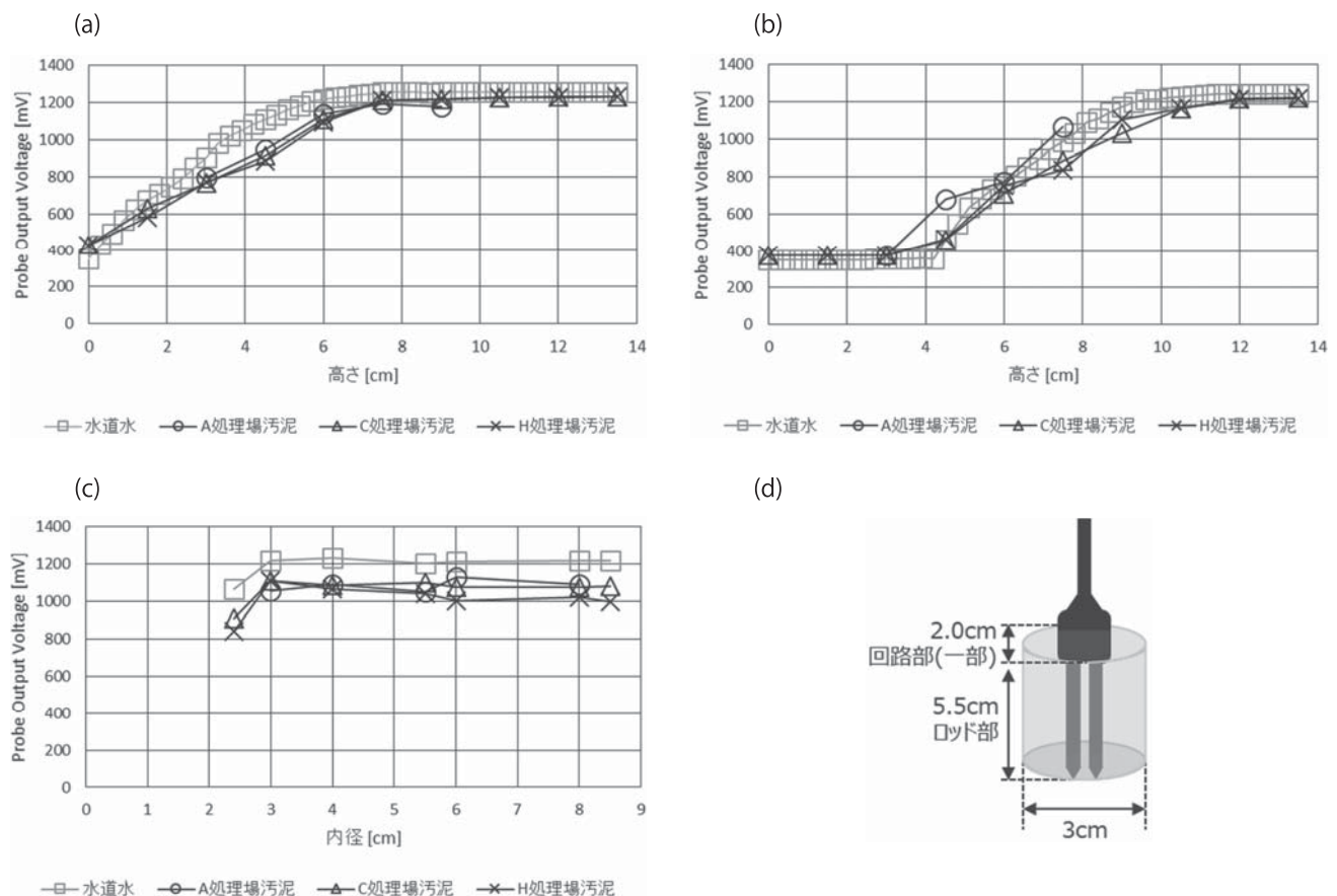
(a : Confirmation of Measurable Height (Top) with Sensor Tip Place at 0 cm Height, b : Confirmation of Measurable Height (Bottom) with Sensor Tip Place at 4.5 cm Height, c : Confirmation of Measurable Weigh, d : Minimum Required Area of EC-5 Soil Moisture Sensor)
