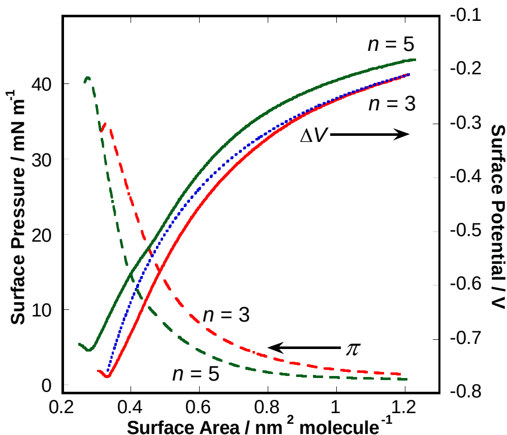
Figure 3. The \pi -A (dashed line) and \Delta V -A (solid line) isotherms of Langmuir monolayers of MA-Rf3 (red) and MA-Rf5 (green) at 15 °C (phase II). The blue dotted line is a calculated density curve.
