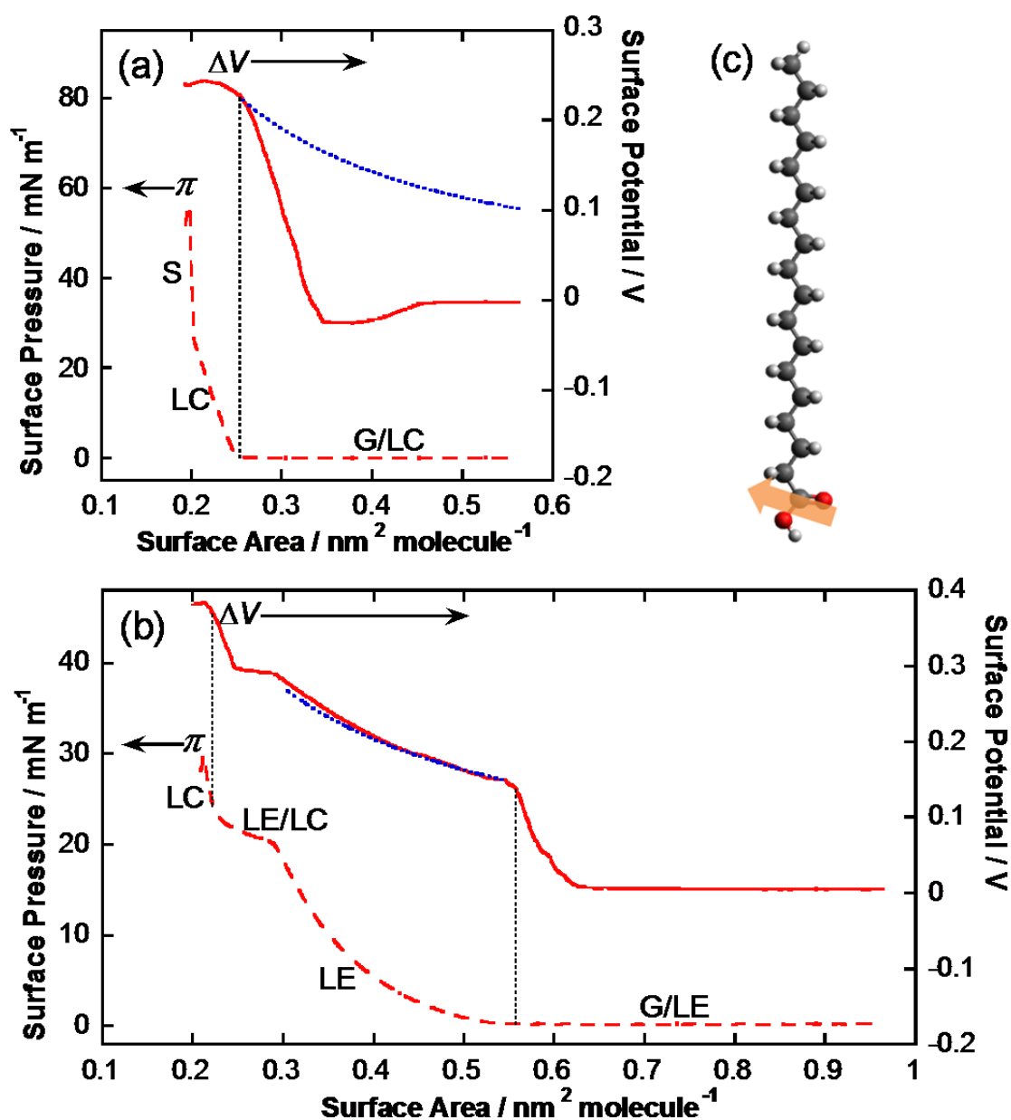
Figure 1. The \pi -A (dashed red line) and \Delta V -A (solid red line) isotherms of a Langmuir monolayer of (a) stearic acid (SA) and (b) myristic acid (MA) measured at 25 °C. The blue dotted line in the panel (a) and (b) is a calculated "density curve" (see the text for detail). (c) A molecular schematic of stearic acid. The orange arrow represents the molecular dipole moment calculated by a quantum chemical calculation.
