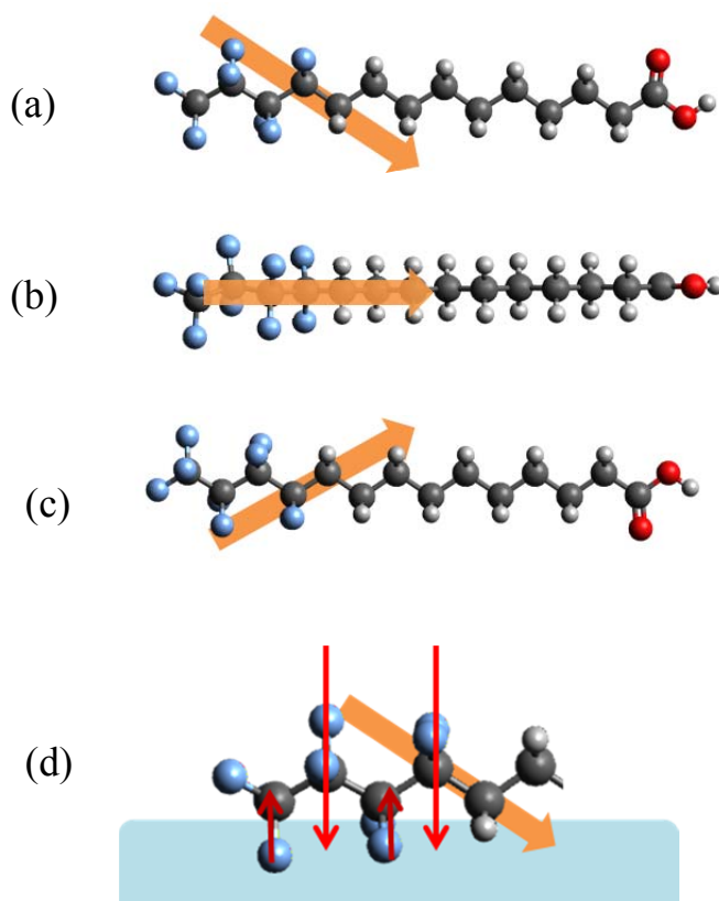
26 Figure 4. (a)~(c) Three different rotational orientations of a lying MA-Rf3 molecule. 27 (d) A schematic view of a dipole-interactive Rf group in the water surface 28 based on the schematic (a). 29 30
