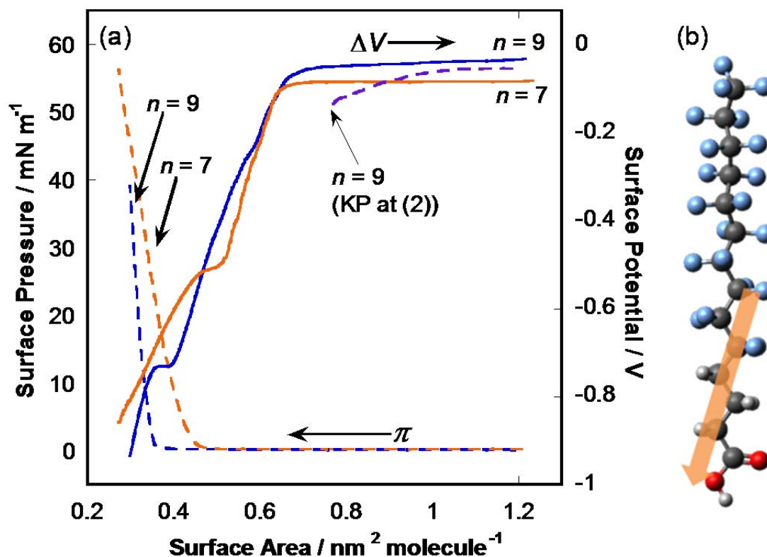
Figure 2. (a) The \pi -A (dashed line) and \Delta V -A (solid line) isotherms of Langmuir monolayers of MA-Rf7 (orange) and MA-Rf9 (blue) at 15 °C (phase II). The \Delta V -A isotherm of MA-Rf9 displayed in purple is measured with the KP at the position of (2) in Chart 1. (b) A molecular schematic of MA-Rf9. The orange arrow represents the molecular dipole moment. The blue atoms are fluorines.
