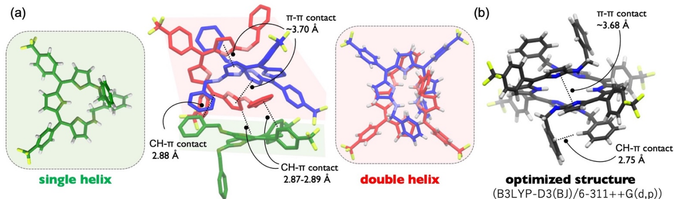
Fig. 2 (a) X-Ray crystal structure of 5 (CCDC 2054819). Red and blue molecules form a double helical structure and green one exists as a monomer. Intermolecular interactions are highlighted. Hydrogen atoms were omitted for clarity in the center. (b) Optimized structure of the double helical structure calculated at the B3LYP-D3(BJ)/6-311++G(d,p) level of theory.
