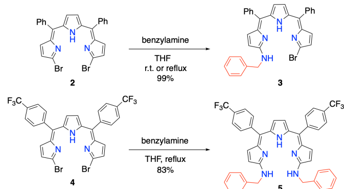
Scheme 1. Synthesis of \alpha,\alpha' -dibenzylaminotripyrrin.
