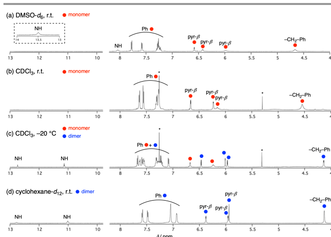
Fig. 1 ^1\text{H} NMR spectra of 5 ; a) in \text{DMSO}-d_6 at rt, b) in \text{CDCl}_3 at rt, c) in \text{CDCl}_3 at -20^\circ\text{C} and d) in cyclohexane- d_{12} at rt.
