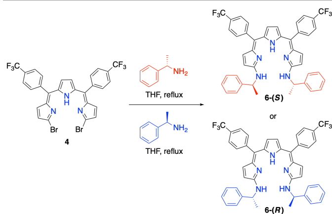
Scheme 2. Synthesis of (S)/(R)-phenylethylamine-substituted-diaminotripyrrin 6 .
