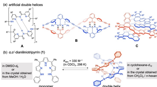
Chart 1. (a) Examples of artificial double helix molecules. (b) An equilibrium of single- and double-helical forms of \alpha,\alpha' -dianilinothripyrrin 1 .
