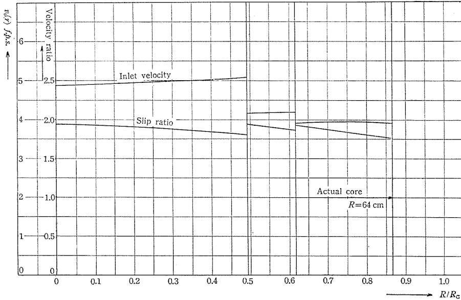
Fig. 5. Inlet velocity and velocity ratio as the functions of radial location, EBWR 50 MW.
