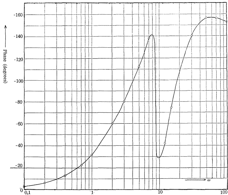
Fig. 11. Feedbacks transfer function, EBWR 50 MW.
