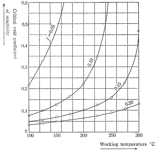
Fig. 1. Critical void coefficient of reactivity as a function of saturated temperature of the moderator, \frac{\partial K}{\partial t_m} = -2.16 \times 10^{-4}/^{\circ}\text{C} .
