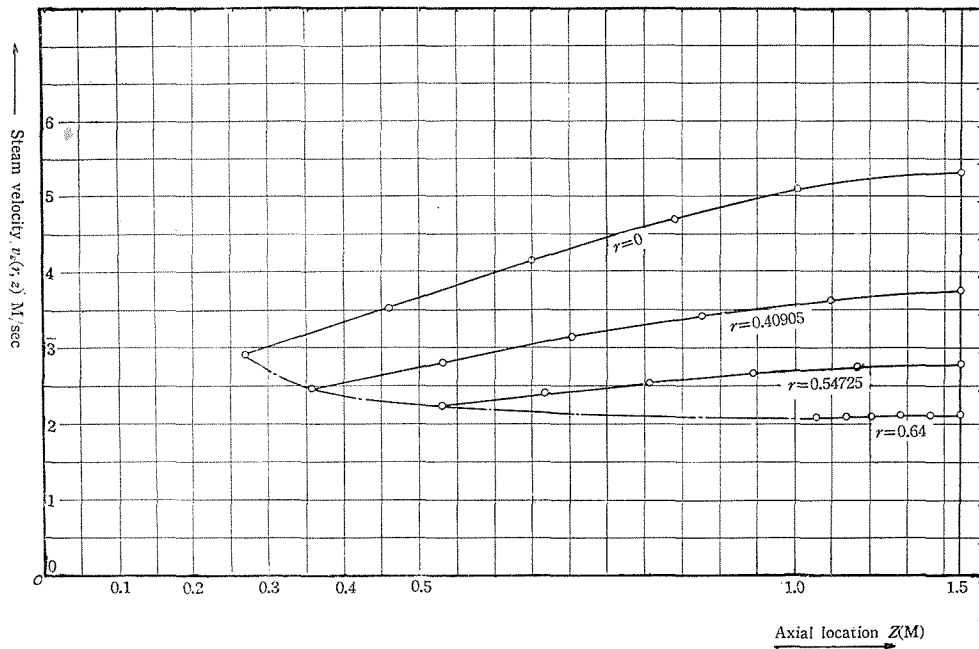
Fig. 8. Spatial distribution of steam flow velocities, EBWR 50 MW.
