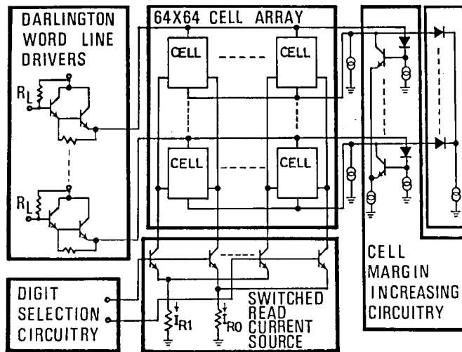
Fig. 3.6. Outline of circuit diagram of the 4K-bit RAM.
