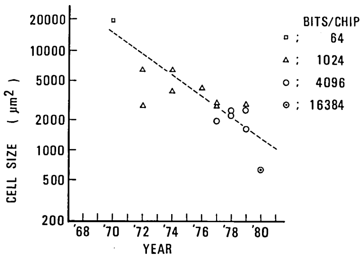
Fig. 2.2. Cell size evolution.
