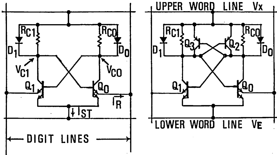
Fig. 2.6. Parallel diode cell. Fig. 2.7. Variable impedance cell.
