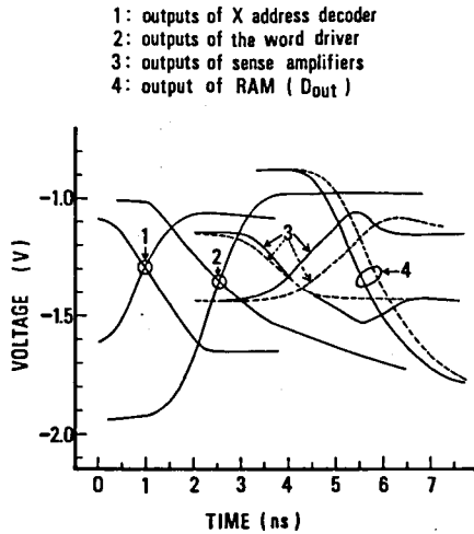
Fig. 4.8. Simulated waveforms in X address access. X address inputs are applied at the time of 0 ns. (Solid line: collector-dot type sense amplifiers. Dotted line: wired-OR emitter follower type ones.)
