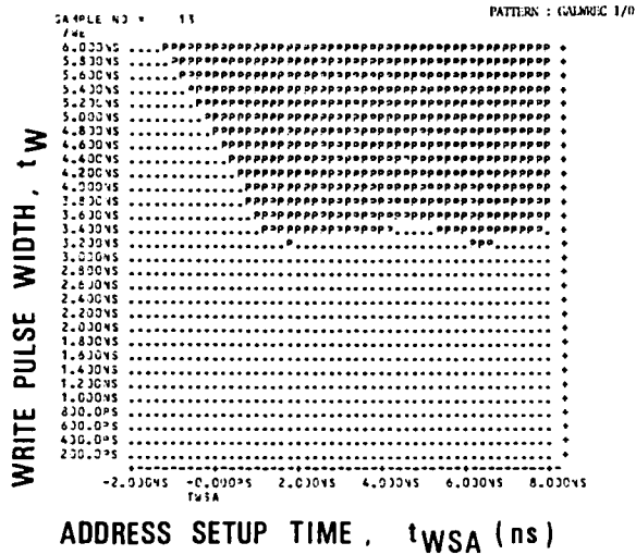
Fig. 2. (a) The 1K-bit RAM's write pulse width t_W vs. address setup time. ( t_W : Writing into any cell can be performed with a longer pulse than t_{WS} .)
