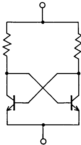
Fig. 2.4. Basic cell circuit.
