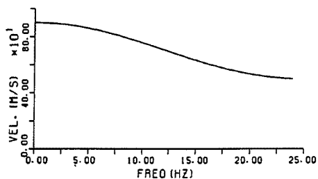
Fig. 5. Dispersion curve.
