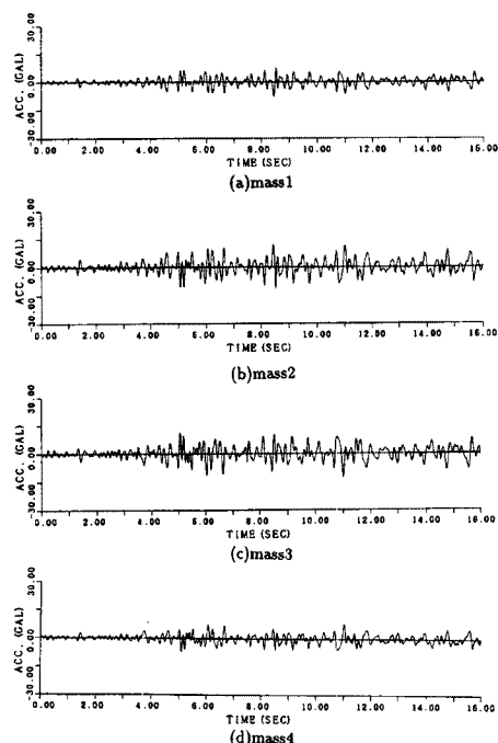
Fig. 14. Identified input accelerations.
