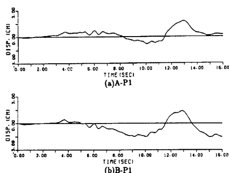
Fig. 13. Response displacement.
