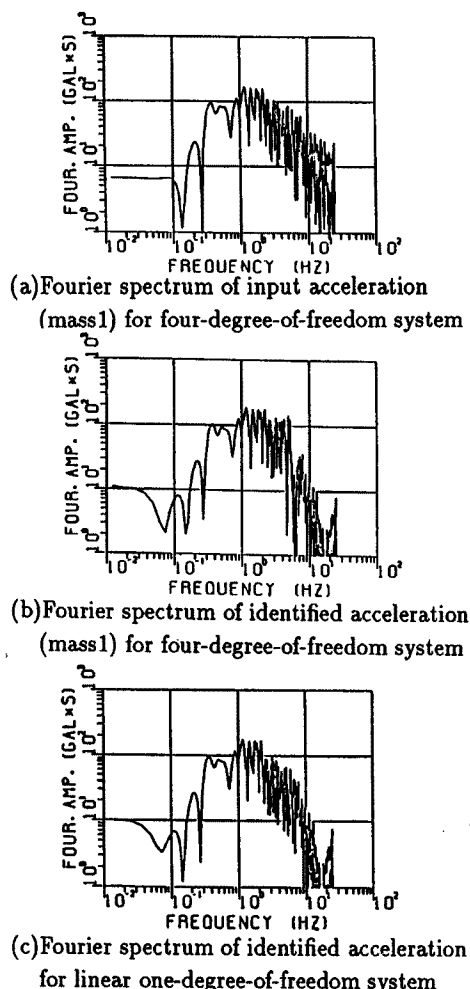
Fig. 9. Comparison of Fourier spectrum.
