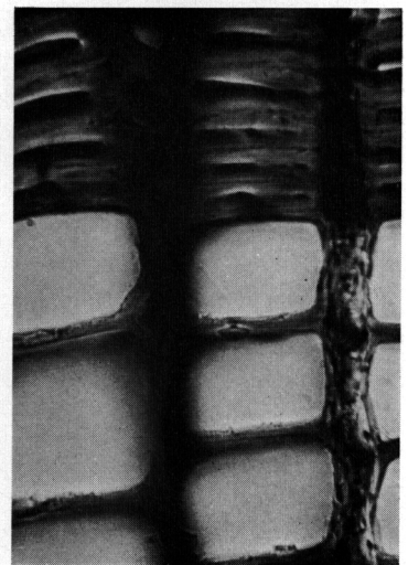
Photo 2. Mature wood tracheids showing higher coloring intensity in radial wall than tangential wall. Momi in green wood.
