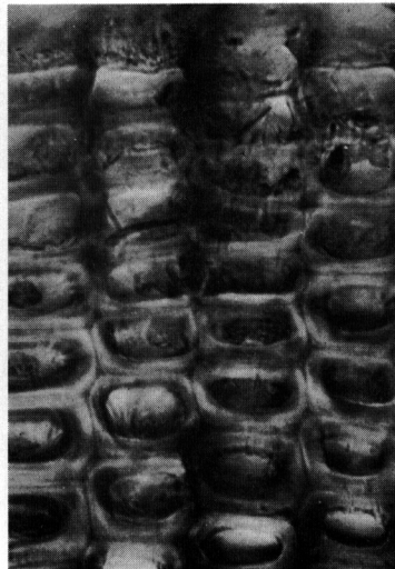
Photo 1. The outermost annual ring stained with phloroglucinol-hydrochloric acid, showing different coloring in radial and tangential walls during wood formation. Momi ( Abies firma ) in green late wood.
