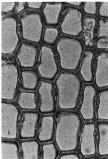
Photos 6-a (left) and 6-b (right). Early wood tracheids of Sugi unstained (a) and stained (b).
