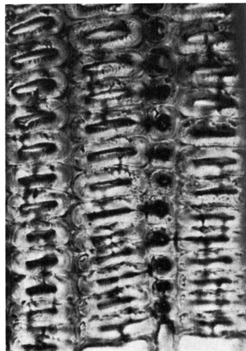
Photos 3 (left) and 4 (right). Transverse sections from air-dried wood of Momi (Photo 3) and Sugi (Photo 4), showing higher coloring intensity in radial wall than tangential.
