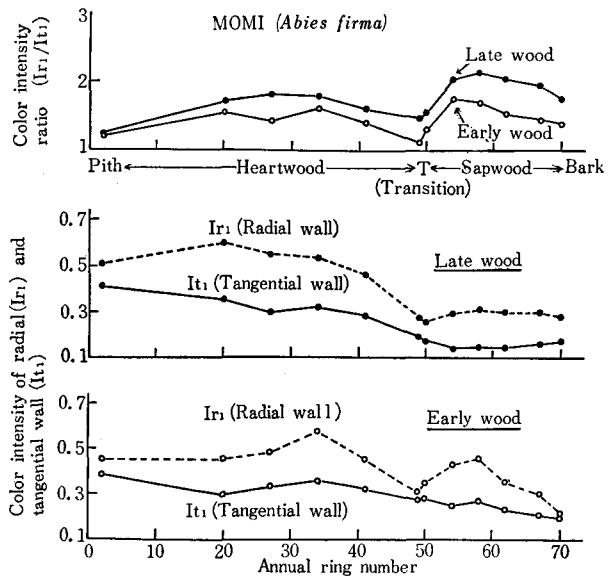
Fig. 4. Variations of color intensity of radial ( I_{r1} ) and tangential walls ( I_{t1} ), and the ratio I_{r1}/I_{t1} from pith to bark—Momi ( Abies firma ), air-dried wood tracheids.
