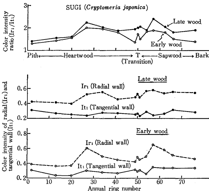
Fig. 3. Variations of color intensity of radial ( I_{r1} ) and tangential walls ( I_{t1} ) and the ratio ( I_{r1}/I_{t1} ) from pith to bark Sugi ( Cryptomeria japonica ), air-dried wood tracheids.
