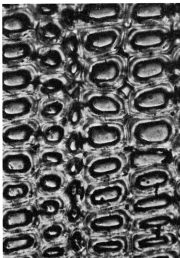
Photos 5-a (left) and 5-b (right). Late wood tracheids of Sugi ( Cryptomeria japonica ) unstained (a) and stained (b) with phloroglucinol-hydrochloric acid. In unstained section (a) similar brightness both in radial and tangential walls is shown. In stained section (b) coloring intensity is higher in the radial wall than in tangential.
