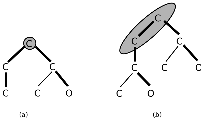
Figure 3.2: Illustration of two kinds of center-rooted trees. The thick lines represent one of the longest paths, and the vertices in circles represent the center.
