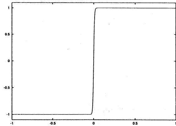
(b) \tanh(100x)
