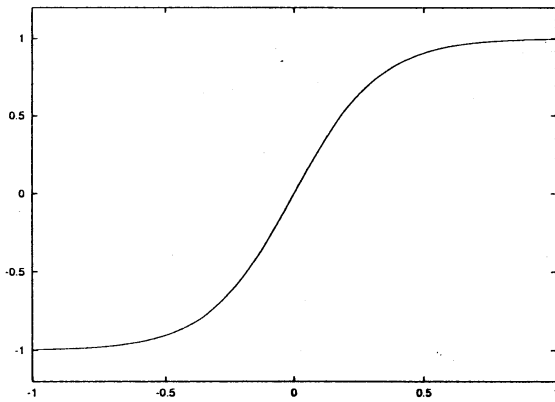
(a) \tanh(3x)
