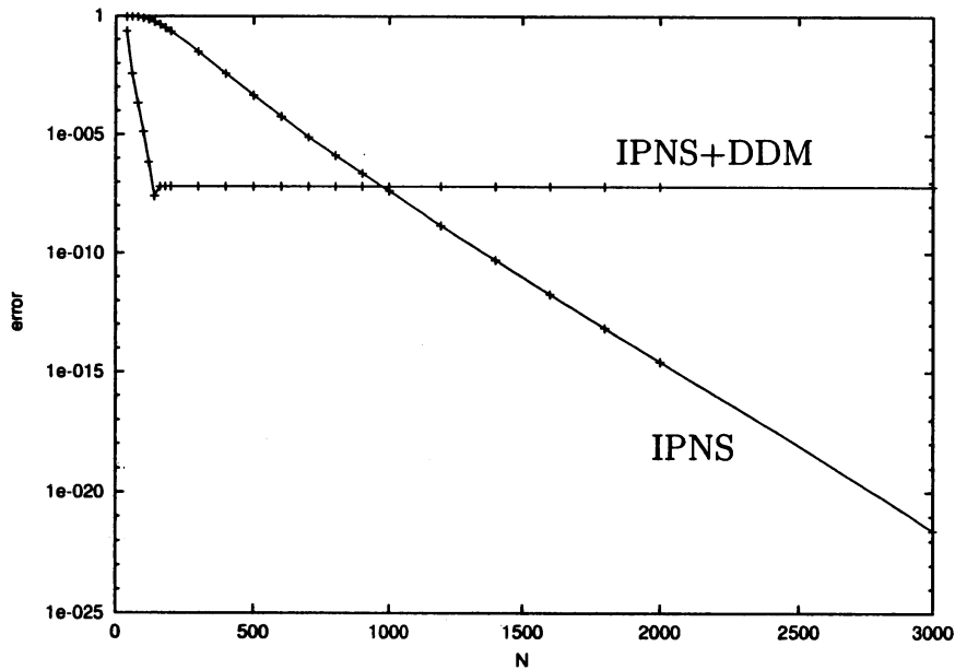
Fig. 2. Behavior of maximum error for Problem 1 with a = 100 . (Quadruple precision, DDM : c = 0.1 , N_1 = N_3 = 10 )
