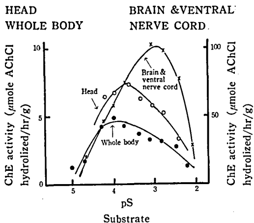
Fig. 1. Activity-pS ( -\log mole of substrate) curves for the enzymatic hydrolysis of acetylcholine chloride in three sources of armyworm enzyme. Reaction conditions; enzyme concentrations, head, 4%, whole body, 10% and brain & ventral nerve cord, 1%, pH adjusted at 7.4 with phosphate buffer. Incubation time, 10 min at 37^\circ\text{C} .
