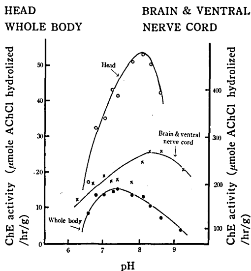
Fig. 4. Variation in ChE activity of 3 sources of armyworm enzyme as a function of pH. The reaction conditions were: substrate concentration for head and whole body homogenates, 2.5 \times 10^{-4} M final, brain & ventral nerve cord, 1.0 \times 10^{-3} M final, enzyme concentrations: head, 4%, whole body, 10%, brain & ventral nerve cord, 1%. Incubation time, 10 min at 37°C. For full explanation see Text.
