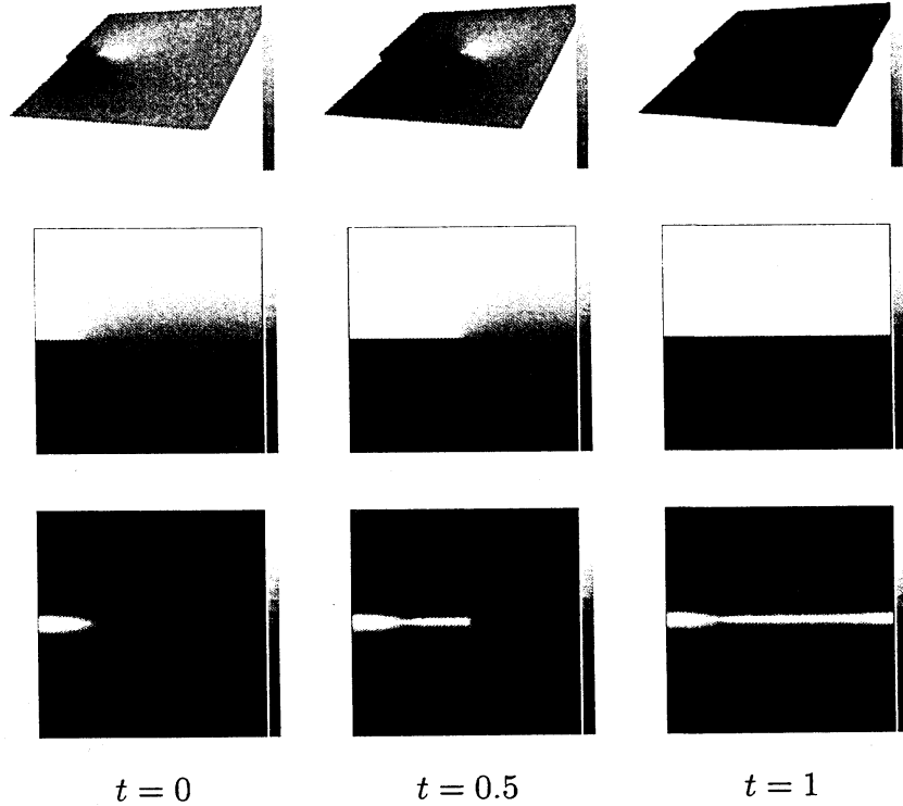
Figure 2: Birdview of u (top), u (middle) and z (bottom).
