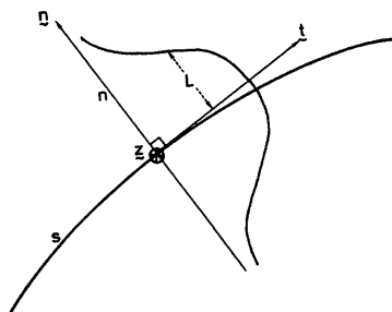
Fig. 2 Ray-centered coordinates (s, n) and basic unit vectors \underline{l} , \underline{n} and \underline{z} after Yomogida.
