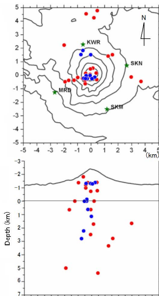
Fig. 4 Hypocentral distribution of volcano-tectonic earthquakes at Sinabung during the period from September 6 to 7. Red and blue dots indicate hypocenters before and after the explosive eruption at 00:23 on September 7.
