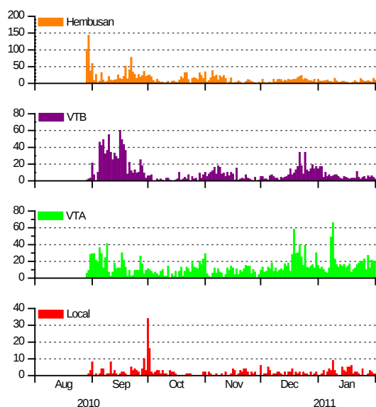
Fig. 3 Daily number of types of volcanic earthquake during the period from August 29, 2010 to January 31, 2011.
