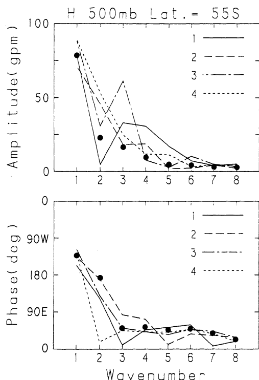
Fig. 7 Amplitude and phase of the stationary height wave along 55^{\circ}\text{S} in Fig. 6. Average in the whole period is denoted by dot and those in the sub-period by four different lines.
