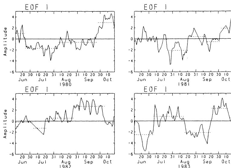
Fig. 15 Time-variation of amplitude A_1 for E_1 defined in Fig. 14. Dotted lines denote averages in each sub-period.
