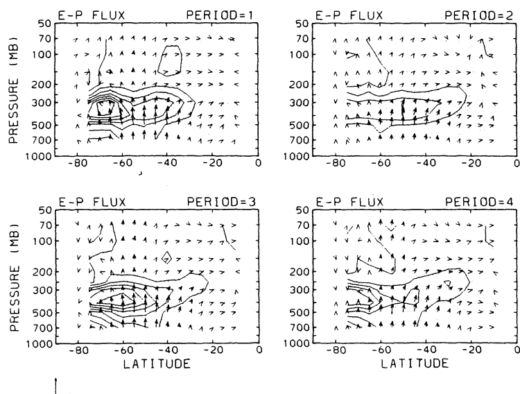
Fig. 10 Latitude-height sections of the E-P flux \bar{F} and wave driving \bar{D}_F for the four periods. Contour interval of \bar{D}_F is 2.5 \times 10^{-5} \text{ ms}^{-2} ; negative values are shaded. Reference arrow shows 1.0 \times 10^9 \text{ kg s}^{-2} for horizontal direction and 1.0 \times 10^9/c ( c = 317 ) \text{kg s}^{-2} for vertical direction. (See text for the scaling).
