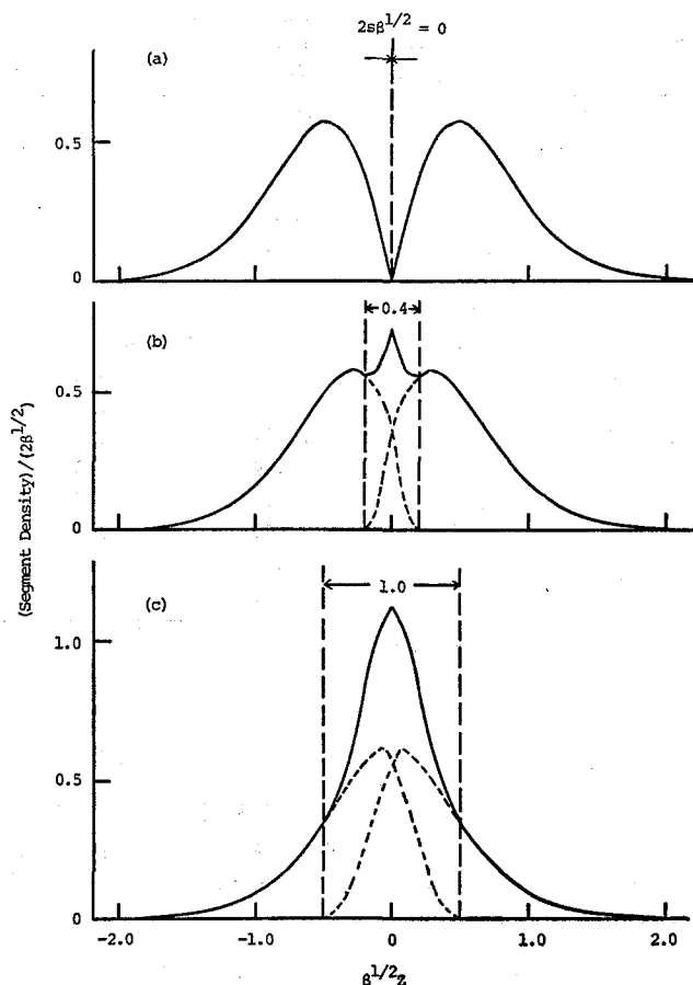
Fig. 2. Density distribution of segments in 'segregation' model with N_A=N_B=N , b_A=b_B=b and s_A=s_B=s : The thickness of the A - B intermixing phase 2s is (a) 0, (b) 0.4\beta^{-1/2} and (c) 1.0\beta^{-1/2} ; \beta = 3/(2Nb^2) . Broken curves refer to individual blocks.
