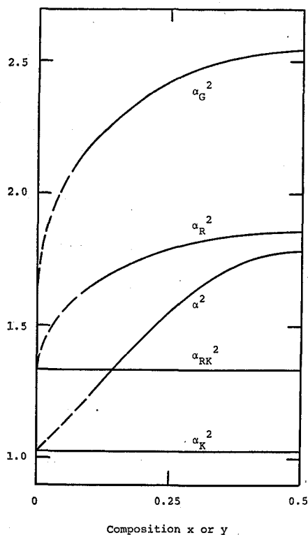
Fig. 4. Plots of dimensional parameters of 'segregation' model with s_A = s_B = 0 and b_A = b_B = b versus composition x or y ; \alpha 's are as in Figure 3.
