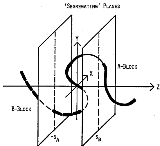
Fig. 1. Schematic representation of 'segregation' model. The A-B junction point is at Z=0 . The A- and B-blocks are restricted from entering the regions Z < -s_A and Z > s_B , respectively.
