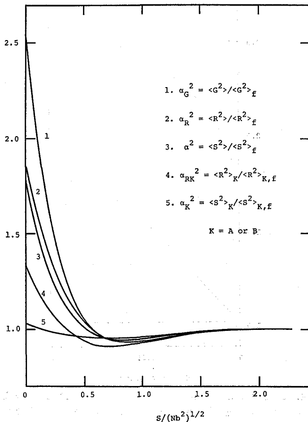
Fig. 3. Plots of dimensional parameters of 'segregation' model with N_A=N_B=N , b_A=b_B=b and s_A=s_B=s versus s/(Nb^2)^{1/2} ; \alpha 's are as indicated in the figure.
