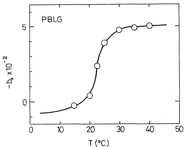
(a) Temperature dependence of b_0 in a 75.0 vol%-DCA-25.0 vol%-DCE mixture for PBLG (Sample C-1).
