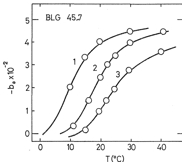
Fig. 7. Temperature dependence of b_0 in DCA-DCE mixtures with various solvent compositions for PBGL copolypeptide (Sample C-4, 45.7 mol% BLG); 1) 58.8 vol%-DCA-41.2 vol%-DCE, 2) 61.5 vol%-DCA-38.5 vol%-DCE, and 3) 64.3 vol%-DCA-35.7 vol%-DCE mixture.
