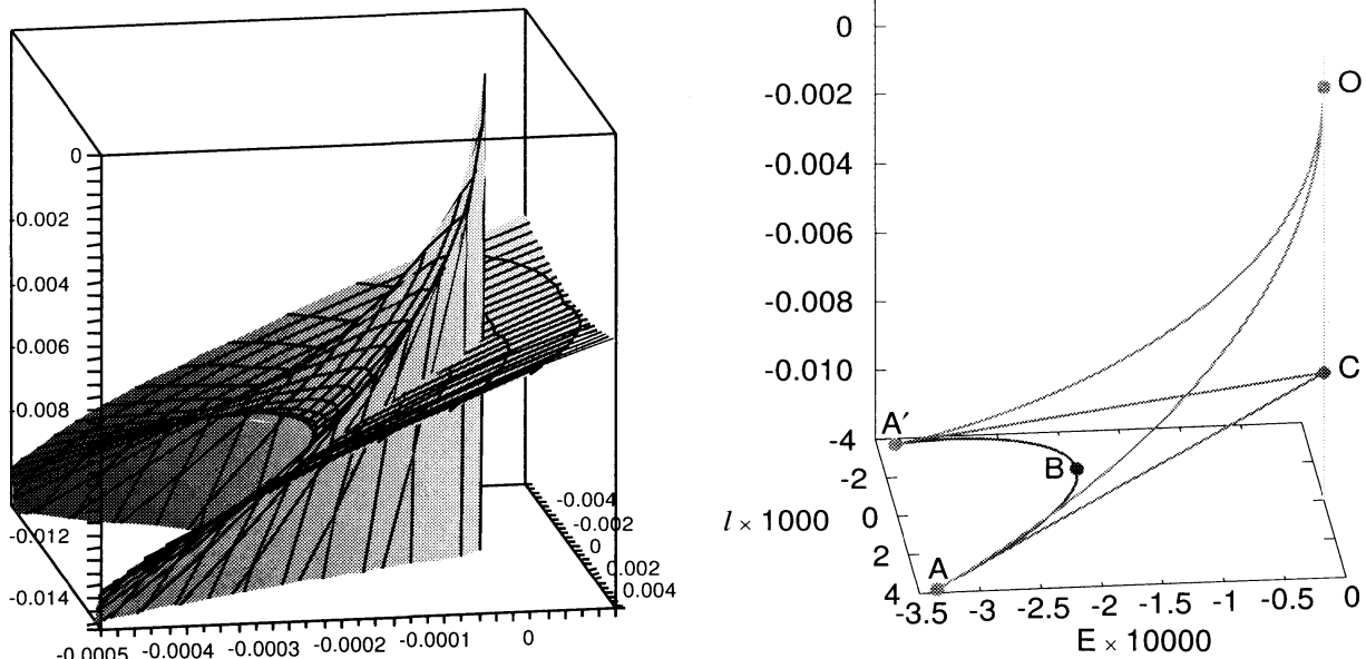
Figure 15: Essential part of the three-dimensional image of the energy-momentum map for 1 : 1 : 2 resonant swing spring [60]. Two connected components of the inverse image of the energy-momentum map are present in the region ABA'OC of the 3D-bifurcation diagram. See text for further explanations.
