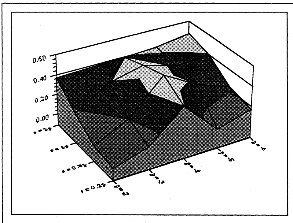
Figure 5. LU decomp rate as a function of time step and precision
