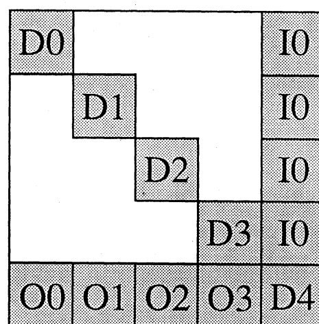
Figure 2. A Boardered Block-Diagonal Matrix
