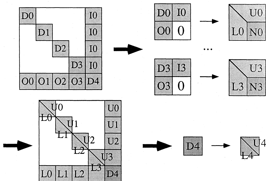
Figure 3. The Block LU Decomposition for a Boardered Block-Diagonal Matrix
