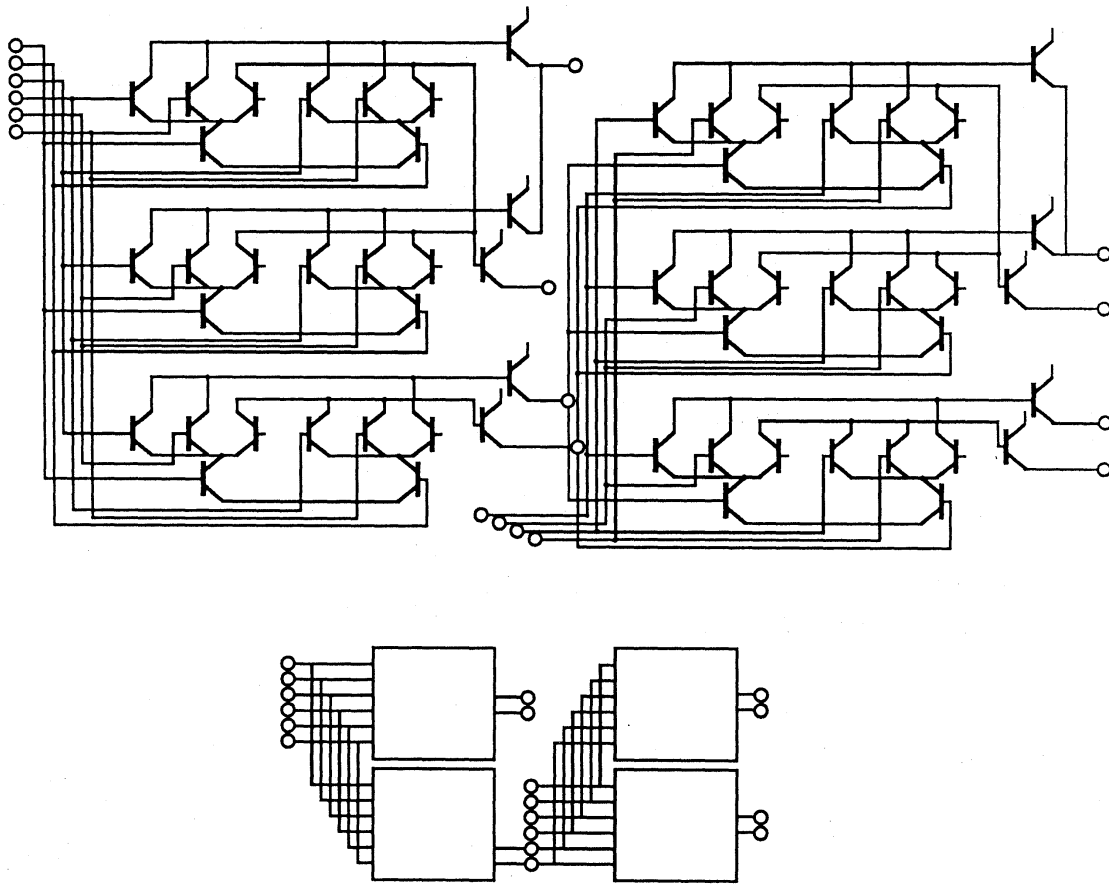
Figure 1. Detailed Circuits and Global Connection
