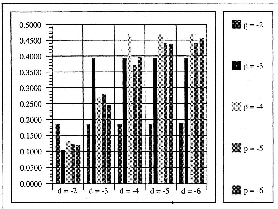
Figure 7 LU decomp rate as a function of \delta_0 and precision
