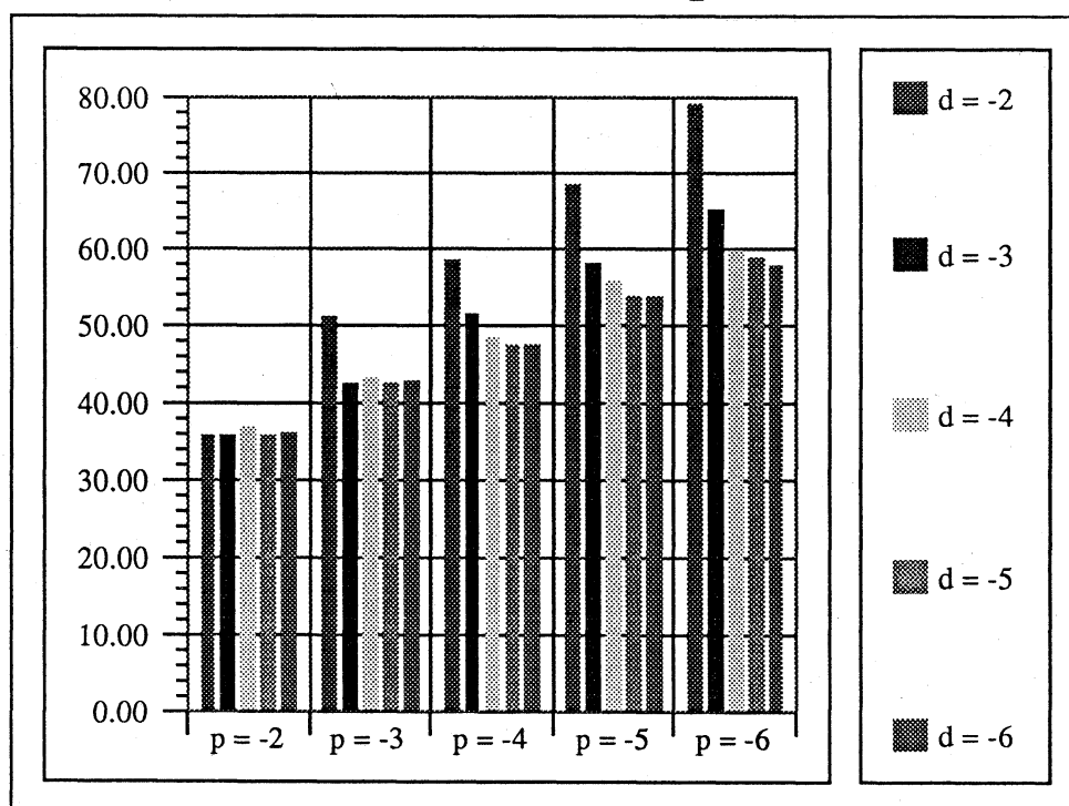
Figure 8. Time as a function of \delta_0 and precision
