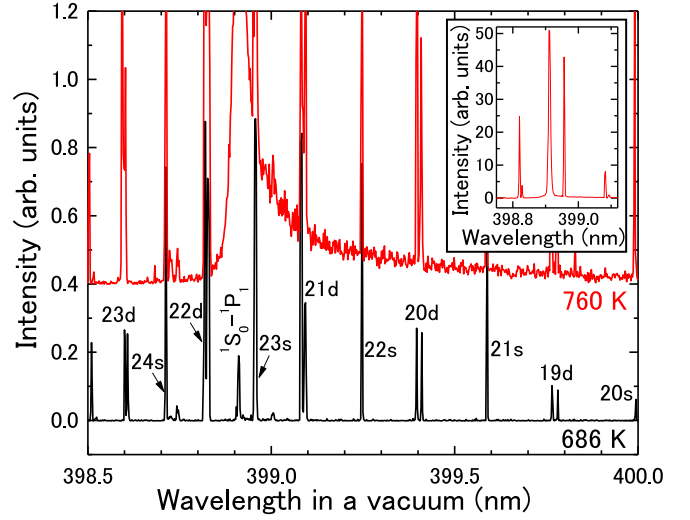
FIG. 2. Excitation spectra of Yb vapors obtained by monitoring the 555.6 nm fluorescence at two different temperatures shown with different offsets. The resonance line at 398.91 nm is the 1S_0 - 1P_1 atomic transition, and the other sharp lines correspond to two-photon excitations to atomic Rydberg states. The labels indicate the assignment of atomic lines, e.g., 24s and 23d refer to the 6s24s 1S_0 and 6s23d 1,3D_2 states, respectively. For a 1,3D_2 doublet the longer-wavelength line is the transition to the 3D_2 state. The broad continuous band observed at 760 K corresponds to the photoassociation of atomic pairs. The inset shows a part of the spectrum at 760 K with a large scale for the vertical axis.
