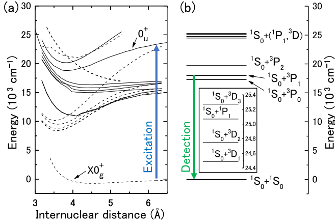
FIG. 1. Molecular and atomic energy-level diagrams. (a) Potential-energy curves of \text{Yb}_2 correlating to the 6s^2 1S_0 + (6s^2 1S_0, 6s6p 1P_1, 6s6p 3P) atomic states. The curves of the X0_g^+ , 0_u^+(1S_0 + 1P_1) , and the other states are traced from the graphs of Ref. [29], Ref. [15], and Ref. [19], respectively. Solid lines are for u states and dashed lines are for g states. Note that the curve of the 0_u^+(1S_0 + 1P_1) state is shifted so that the asymptote coincides with the 1S_0 + 1P_1 atomic level, while the curves of the other excited states are not shifted. (b) Energy levels of Yb atoms. The inset shows the levels around 25000 \text{ cm}^{-1} .
