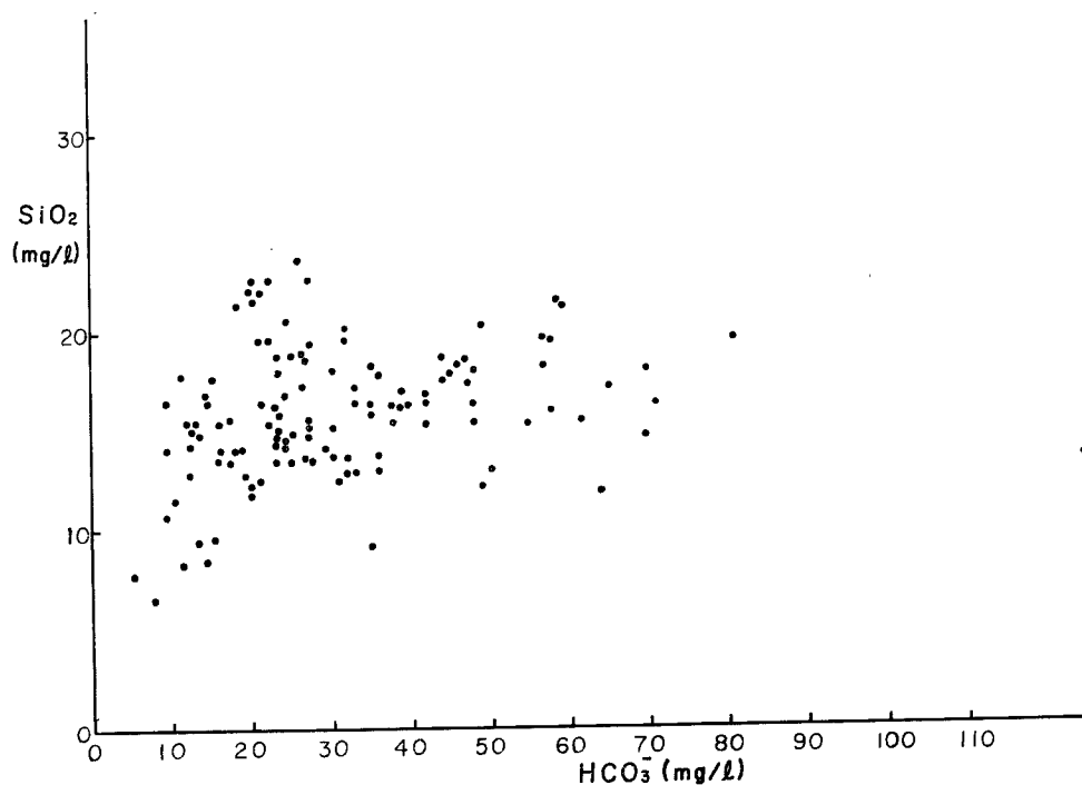
Fig. 3 Relationship between concentrations of \text{HCO}_3^- and soluble silica in Sumiyoshi and Ashiya-gawa areas, Rokko.
