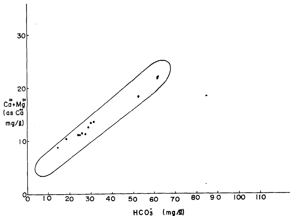
Fig. 22 Relationship between concentrations of \text{HCO}_3^- and \text{Ca}^{2+} + \text{Mg}^{2+} in Rokko-gawa area, Rokko.
