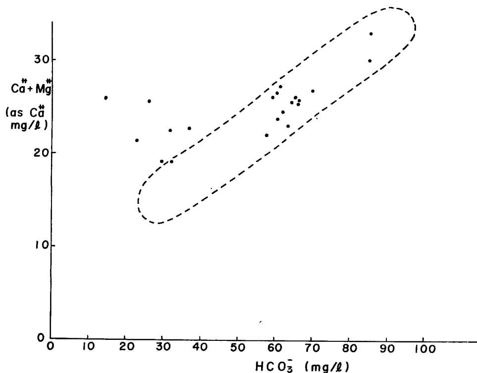
Fig. 13 Relationship between concentrations of \text{HCO}_3^- and \text{Ca}^{2+} + \text{Mg}^{2+} in Uji-gawa (Nodani) area, Rokko.
