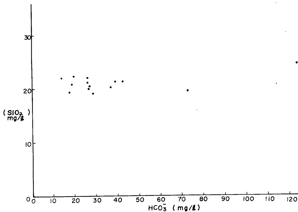
Fig. 6 Relationship between concentrations of \text{HCO}_3^- and soluble silica in Takahashi-gawa area, Rokko.
