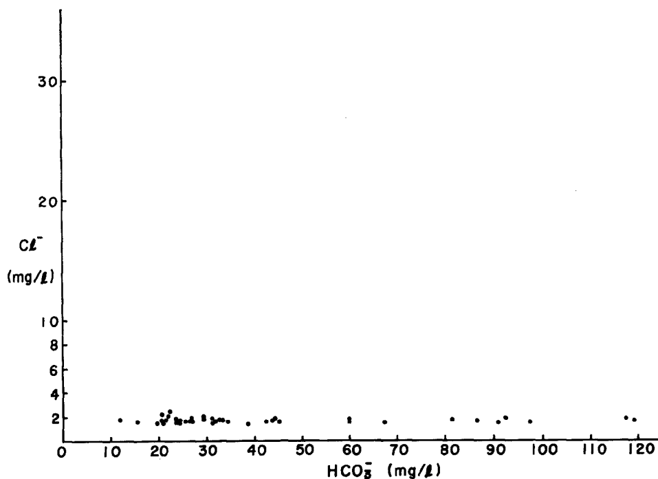
Fig. 38 Relationship between concentrations of HCO_3^- and Cl^- in Ibi-gawa area, Gifu Prefecture.
