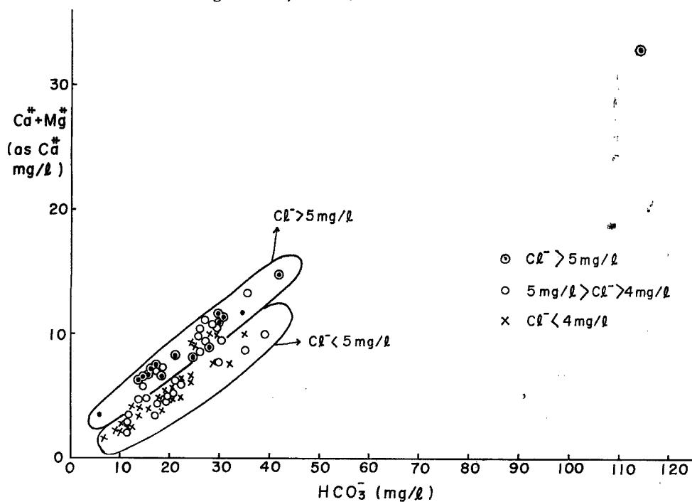
Fig. 25 Relationship between concentrations of \text{HCO}_3^- , \text{Ca}^{2+} + \text{Mg}^{2+} in Okuyama-gawa area, Rokko.
