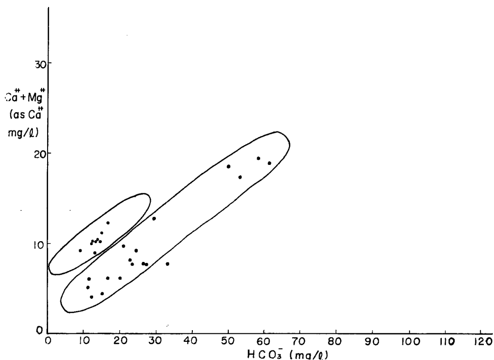
Fig. 7 Relationship between concentrations of \text{HCO}_3^- and \text{Ca}^{2+} + \text{Mg}^{2+} in Tenjo-gawa area, Rokko.
