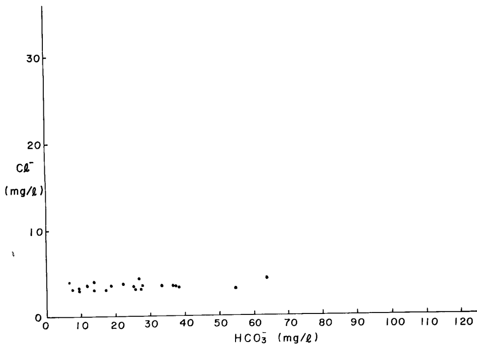
Fig. 35 Relationship between concentrations of \text{HCO}_3^- and \text{Cl}^- in Echi-gawa area, Ibuki.
