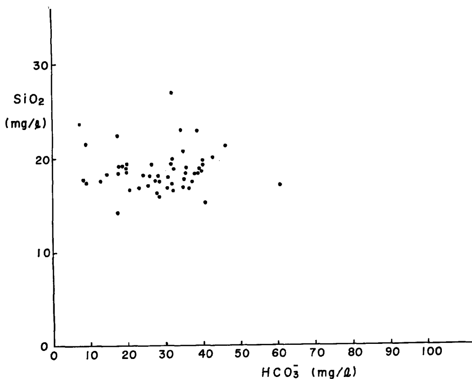
Fig. 21 Relationship between concentrations of \text{HCO}_3^- and soluble silica in Arima-gawa area, Rokko.
