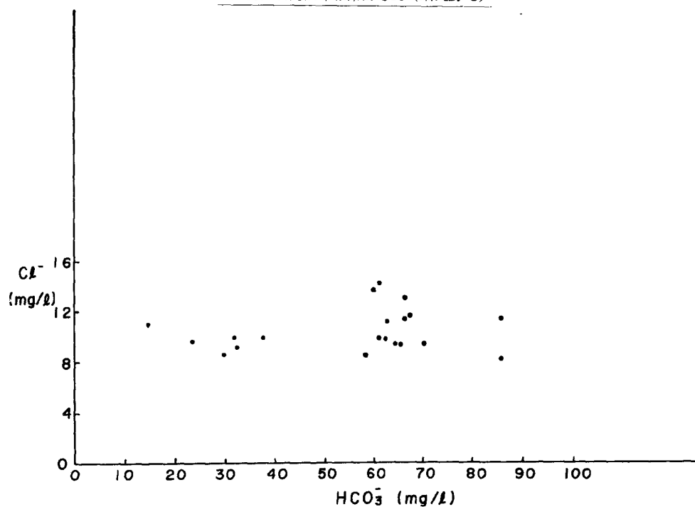
Fig. 14 Relationship between concentrations of \text{HCO}_3^- and \text{Cl}^- in Uji-gawa (Nodani) area, Rokko.
