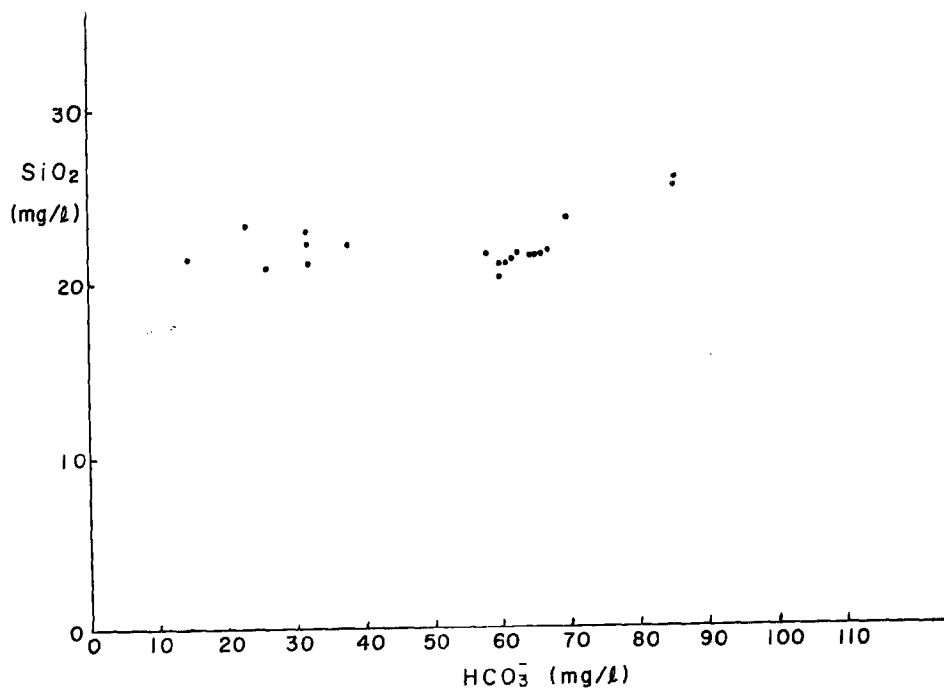
Fig. 15 Relationship between concentrations of \text{HCO}_3^- and soluble silica in Uji-gawa (Nodani) area, Rokko.
