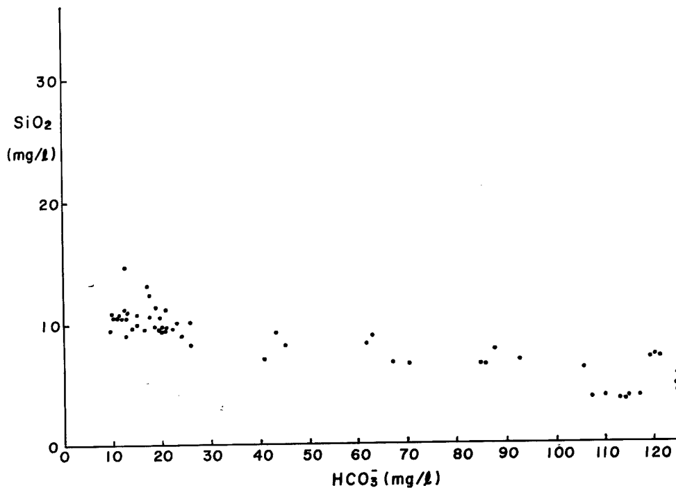
Fig. 33 Relationship between concentrations of \text{HCO}_3^- and soluble silica in Ane- and Kusano-gawa areas, Ibuki.
