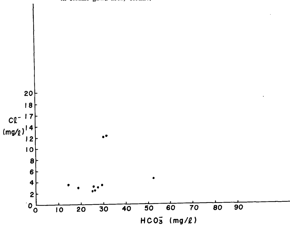
Fig. 23 Relationship between concentrations of \text{HCO}_3^- and \text{Cl}^- in Rokko-gawa area, Rokko.
