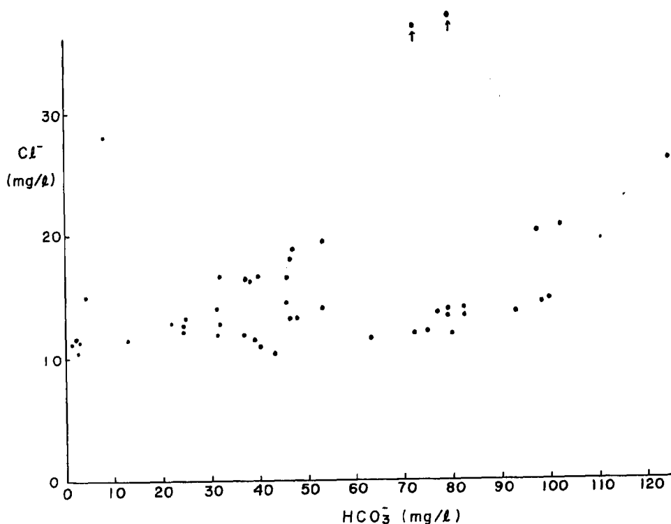
Fig. 17 Relationship between concentrations of \text{HCO}_3^- and \text{Cl}^- in Miyohōji-gawa area, Rokko.
