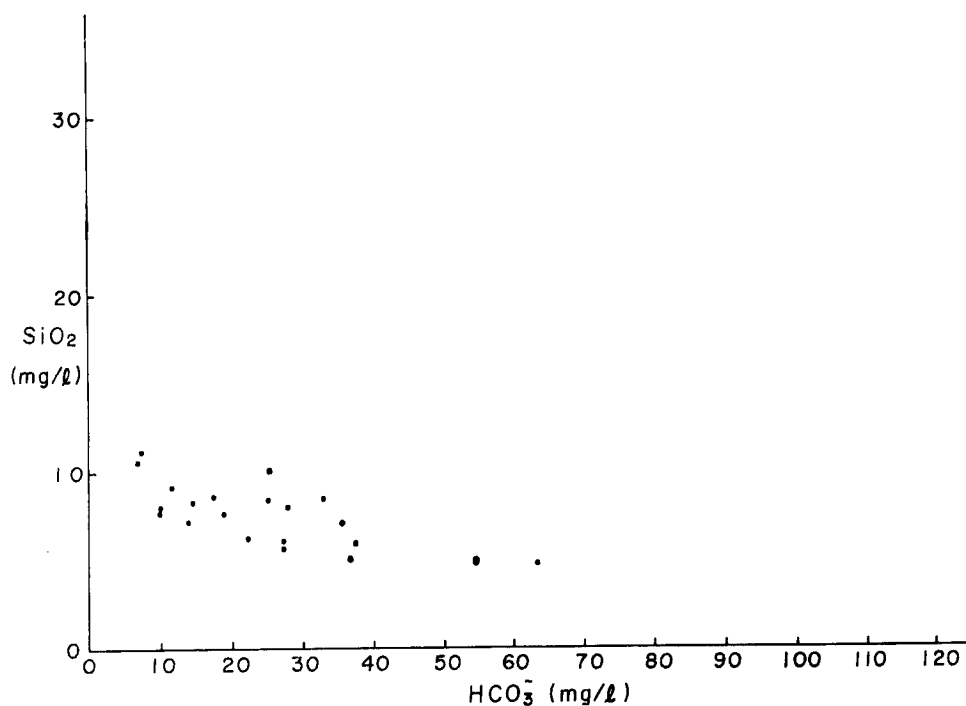
Fig. 36 Relationship between concentrations of \text{HCO}_3^- and soluble silica in Echi-gawa area, Ibuki.
