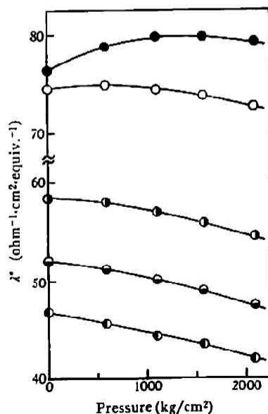
Fig. 1 \lambda^\circ vs. pressure at 25°C ●: \text{Cl}^- , ○: \text{NH}_4^+ , ◐: \text{MeNH}_3^+ , ◑: \text{Me}_2\text{NH}_2^+ , ◒: \text{Me}_3\text{NH}^+
