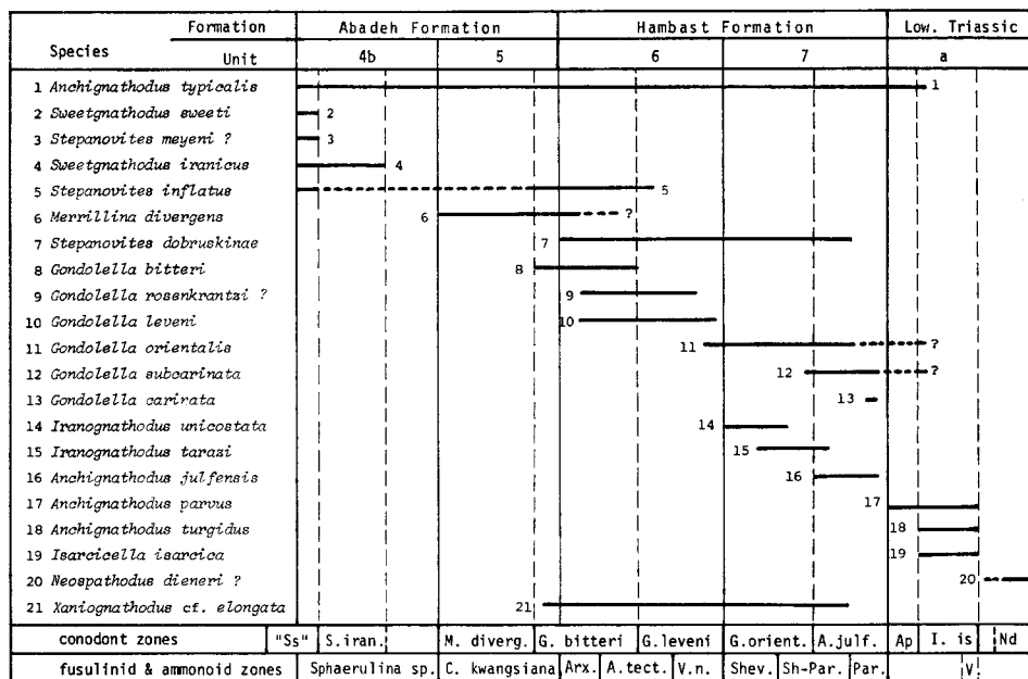
Fig. 22. Range-chart and zones of conodonts compiled from Sections A, C, H and HN.
