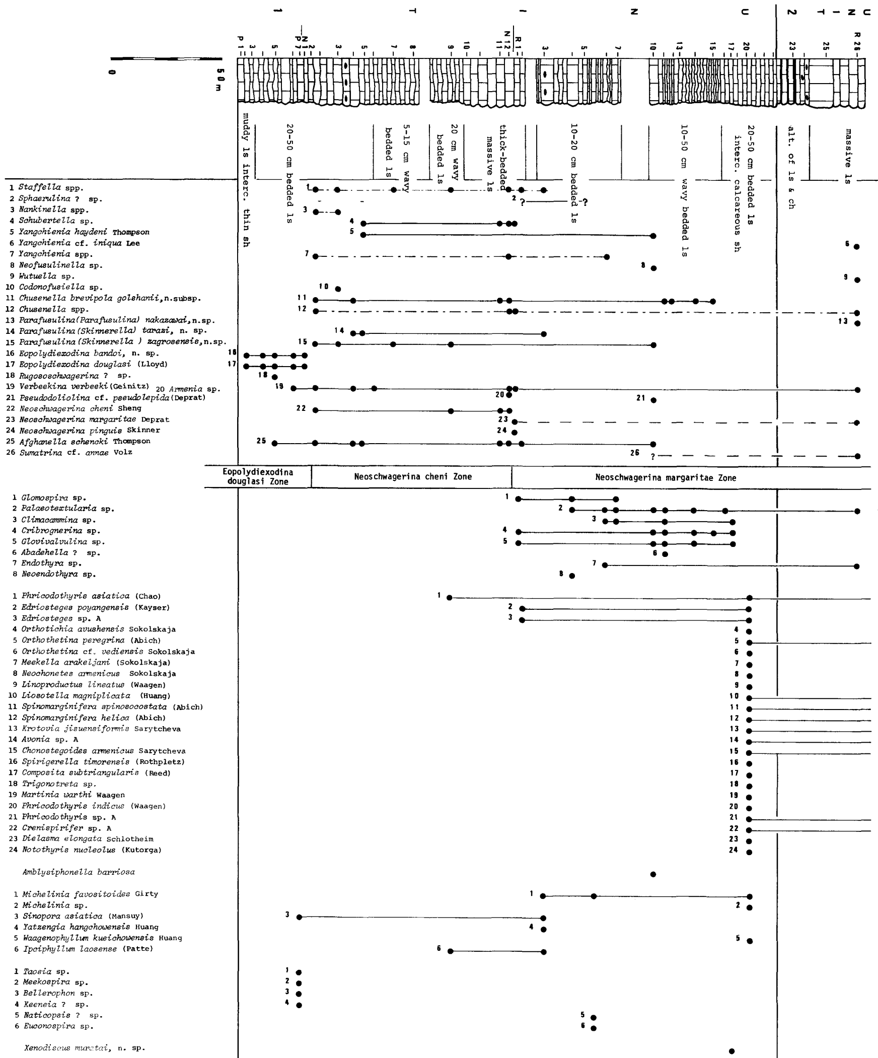
Fig. 5a. Columnar section and range-chart of fossils of Units 1 and 2, Section NR (Sumag).
