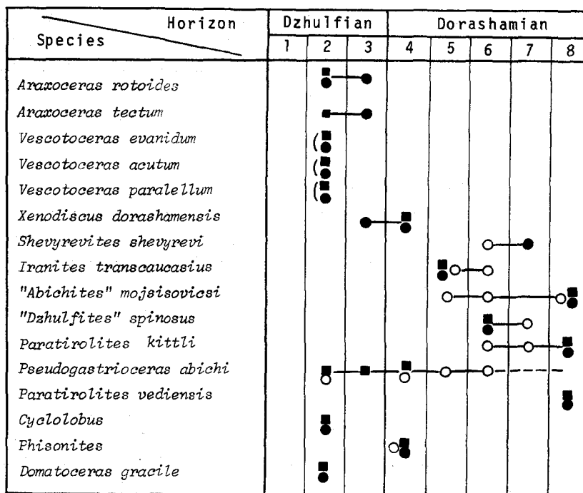
Fig. 9. Stratigraphic occurrence of cephalopod species common to Armenia and Iranian Julfa. Data based on RUZHENTSEV and SARYCHEVA 1965 (solid square), STEPANOV et al. , 1969 (solid circle), and TEICHERT et al. , 1973 (open circle). 1: Araxilevis beds of Armenia or Araxilevis - Orthotetina Zone of Julfa, 2: Araxoceras - Oldhamina beds or Pseudogastriceras - Permophrycodothyris Zone, 3: Vedioceras - Haydenella beds or Haydenella - Pseudowellerella Zone, 4: Phisonites - Comelicania beds or Phisonites Zone, 5: Tompophiceras beds or Tompophiceras (= Iranites ) Zone, 6: Dzhulfites beds or Dzhulfites Zone, 7: Shevyrevites beds or Shevyrevites Zone, 8: Paratirolites beds or Paratirolites Zone.
