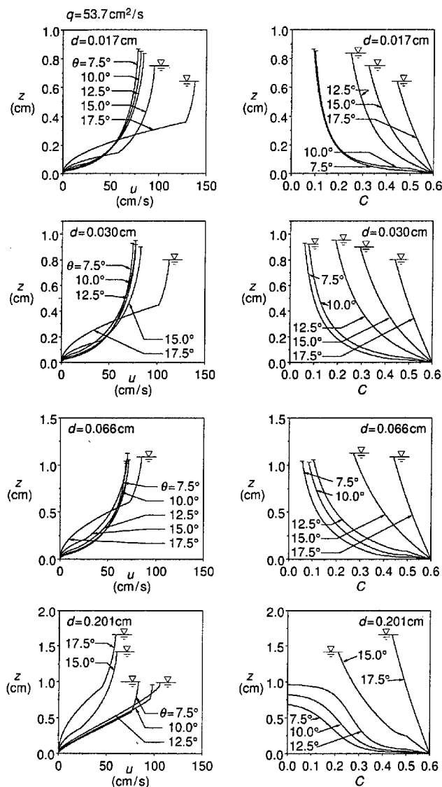
Fig. 5 Solids and velocity distributions under different particle size and channel slope
