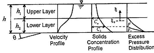
Fig. 3 Structure of the general inertial debris flow
