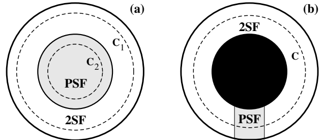
FIG. 2. Different geometries of PSF-2SF interfaces. (See discussion in the text.)
