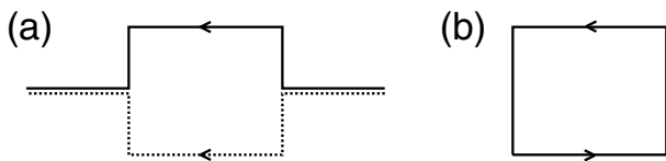
FIG. 1. (a) Unbinding fluctuations of two coupled world lines of the two-component system. (b) The single-loop effective representation. World lines of different species are depicted as solid and dotted lines, respectively.
