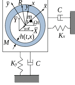
Figure 1: Sketch of the basic configuration, with definition of the space-fixed coordinate system (\bar{X}, \bar{Y}) , the rotating (rotor-fixed) coordinate system (\bar{x}, \bar{y}) , and some of the fundamental symbols.
