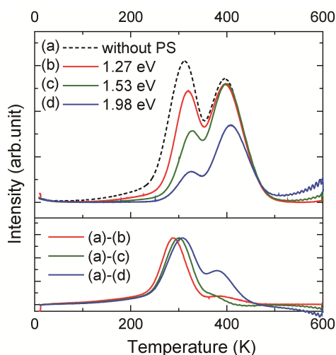
Fig. 5. TSL glow curve measured 1 h after 254 nm excitation for 5 min at 10 K (a) and TSL glow curves measured after 254 nm excitation for 5 min and subsequent photostimulation at 10 K for 1 h by (b) 977 nm (1.27 eV), (c) 808 nm (1.53 eV) and (d) 625 nm (1.98 eV) (upper figure) excitations. Curves in lower figure are each subtraction curves from the curve (a), normalized with respect to the difference measured for peak (I) intensity.
