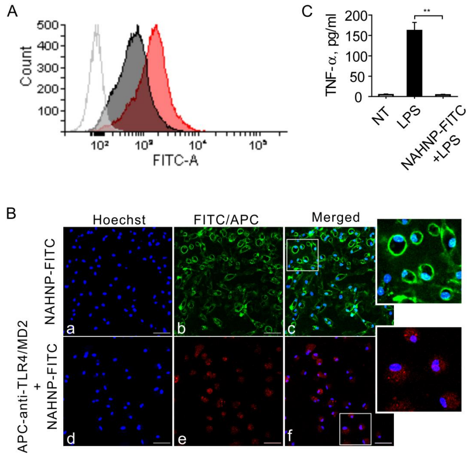
Fig. 7. Evaluation of binding of nanoparticles to TLR4/MD2 receptor complex.
