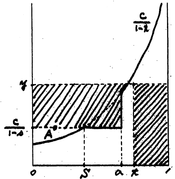
Case (2d): x \geq a, \frac{c}{1-a} \leq y \leq \frac{c}{1-x}
