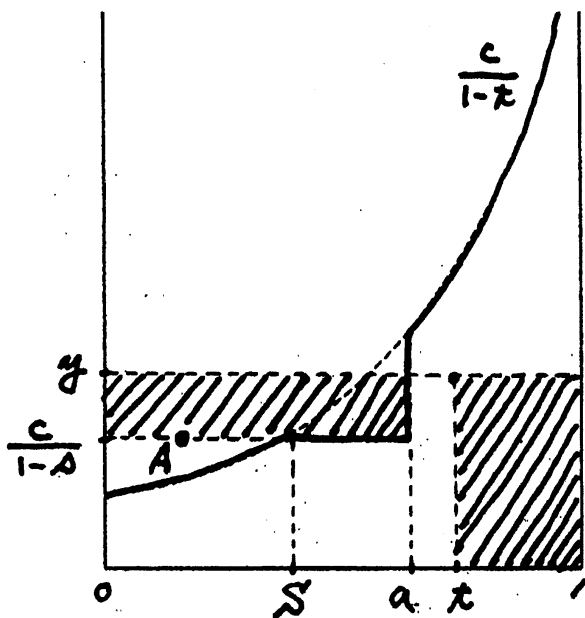
Case (2c): x \geq a, \frac{c}{1-a} \leq y < \frac{c}{1-x}
