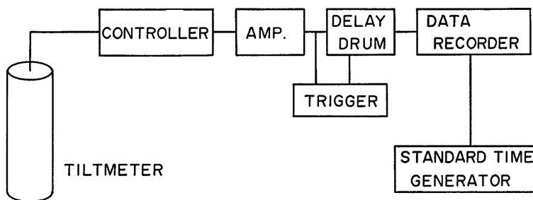
Fig. 3 Block diagram of the observation system.
