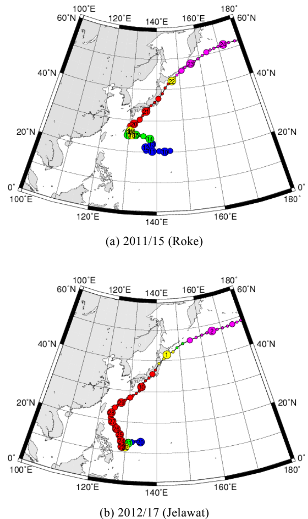
Fig. 2 Track of typhoon (from Digital Typhoon Data)
