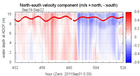
Fig. 7 Contours of north-south velocity component measured by ADCP (Typhoon 2011/15)
