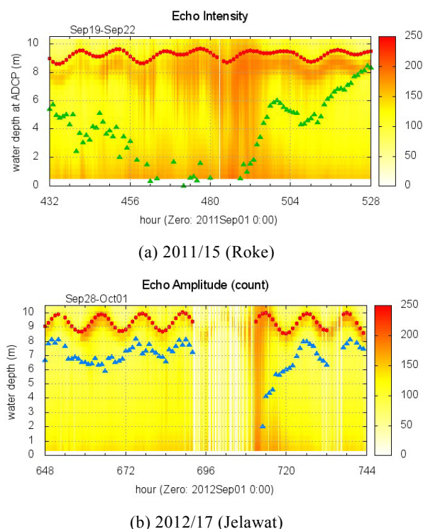
Fig. 8 Contours of echo intensity (including depth related to wave height)
