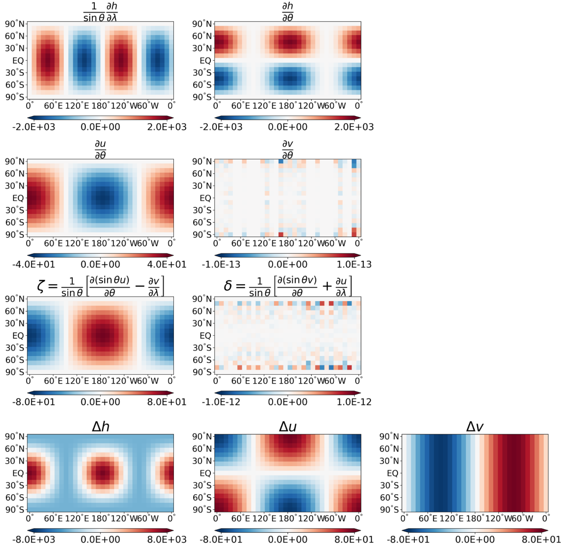
Fig. 2 Differentiation using Fourier transforms. Variables are the gradient, latitudinal derivative of wind, vorticity, divergence, scalar Laplacian, and vector Laplacian (from top to bottom). The horizontal resolution is the same as in Fig. 1.
