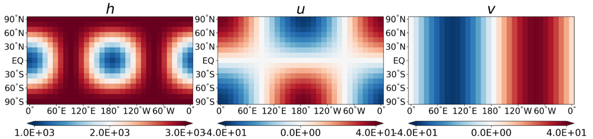
Fig. 1 Input fields of Geopotential height, u-wind, and v-wind (from left to right). The horizontal resolution is 17 grid points in the meridional direction and 32 grid points in the zonal direction.
