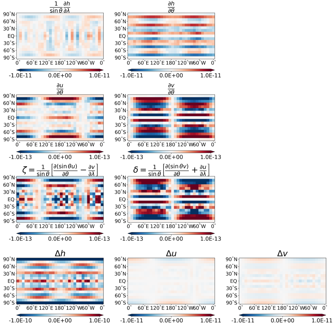
Fig. 4 As in Fig. 3, except that the method used here is the spherical harmonic transform.
