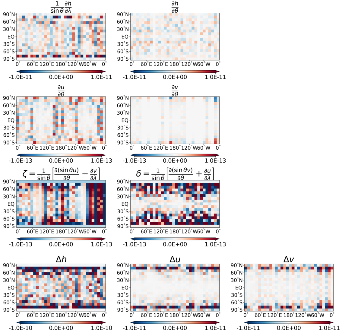
Fig. 3 As in Fig. 2, except that this figure shows the error to the analytical solution, obtained using the Fourier transform method.
