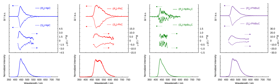
Figure 6. CPL (top), g_{lum} (middle), and PL (bottom) spectra of NpC , PhC , NpBu 2 C , and PhtBuC in the dilute CHCl 3 ( 1.0 \times 10^{-5} M for CPL and 1.0 \times 10^{-6} M for PL). Excitation wavelength was 300 nm, 350 nm, 300 nm, and 314 nm for NpC , PhC , NpBu 2 C , and PhtBuC , respectively.
