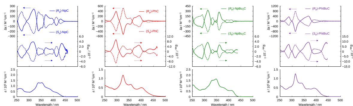
Figure 4. CD (top), g_{abs} (middle), and UV-vis absorption (bottom) spectra of NpC , PhC , NpBu 2 C , and PhtBuC in the dilute CHCl 3 ( 1.0 \times 10^{-5} M).
