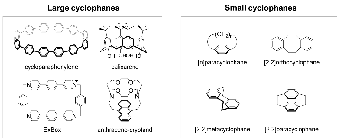
Figure 1. Cyclophane families.
