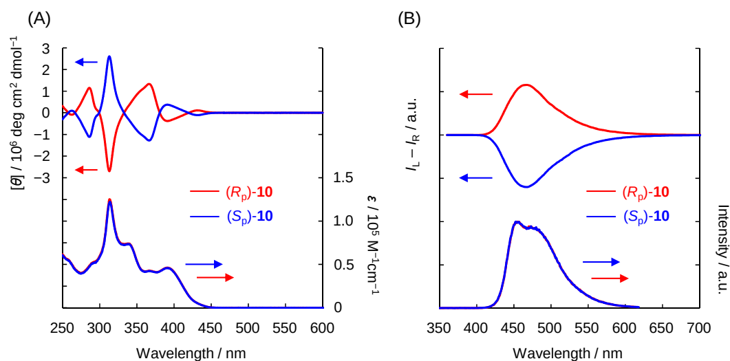
Figure 3. (A) UV-vis absorption and CD spectra of ( R p )- and ( S p )- 10 in CHCl 3 ( 1.0 \times 10^{-5} M) at room temperature. (B) PL and CPL spectra of ( R p )- and ( S p )- 10 in CHCl 3 ( 1.0 \times 10^{-6} M for PL and 1.0 \times 10^{-5} for CPL) at room temperature, excited at 314 nm.
