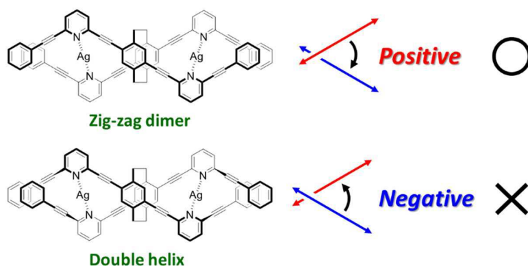
Figure 7. Predicted structures of the Ag(I) complex (S_p)\text{-N-Ph-Ag} by the exciton coupling.
