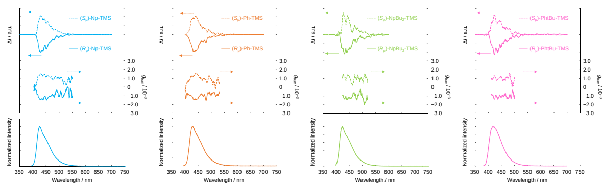
Figure 5. CPL (top), g_{lum} (middle), and PL (bottom) spectra of Np-TMS , Ph-TMS , NpBu 2 -TMS , and PhtBu-TMS in the dilute CHCl 3 ( 1.0 \times 10^{-5} M for CPL and 1.0 \times 10^{-6} M for PL). Excitation wavelength was 300 nm, 350 nm, 300 nm, and 300 nm for NpC , PhC , NpBu 2 C , and PhtBuC , respectively.
