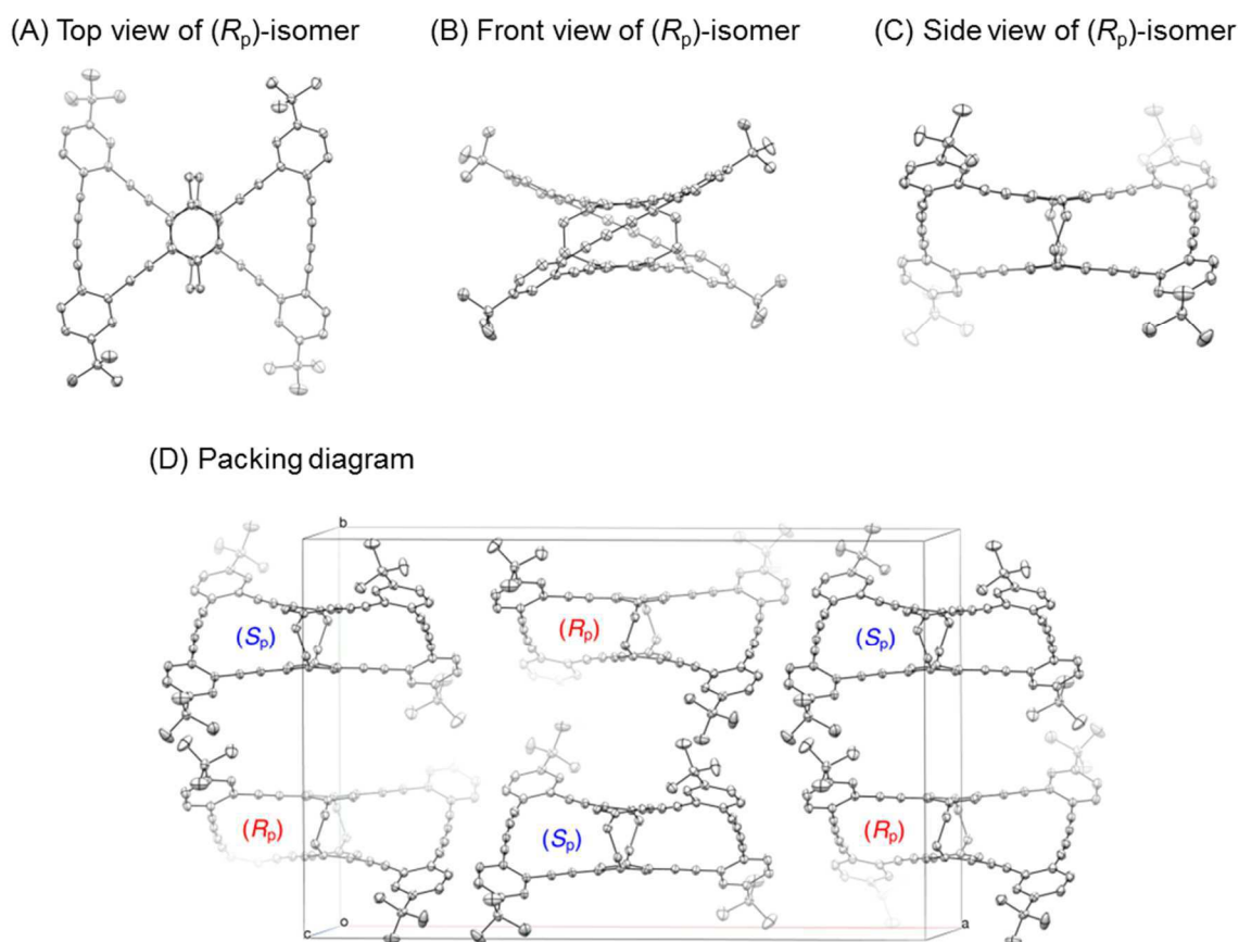
Figure 2. Preliminary X-ray structure of rac - 10 and its packing diagram. Thermal ellipsoids are scaled to the 30% probability level. Hydrogen atoms and solvents are omitted for clarity.
