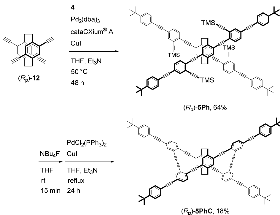
Scheme 3. Synthesis of ( R p )- 5Ph and ( R p )- 5PhC
