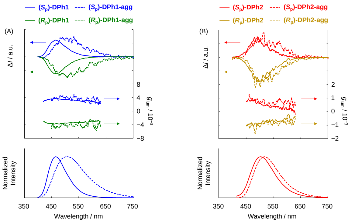
Figure 4. CPL spectra in 1,4-dioxane (solid line) and 1,4-dioxane/H 2 O = 1/99 v/v (dotted line) ( 1.0 \times 10^{-5} M); (A) ( S p )- and ( R p )-DPh1; (B) ( S p )- and ( R p )-DPh2. Excitation wavelength: 350 nm.
