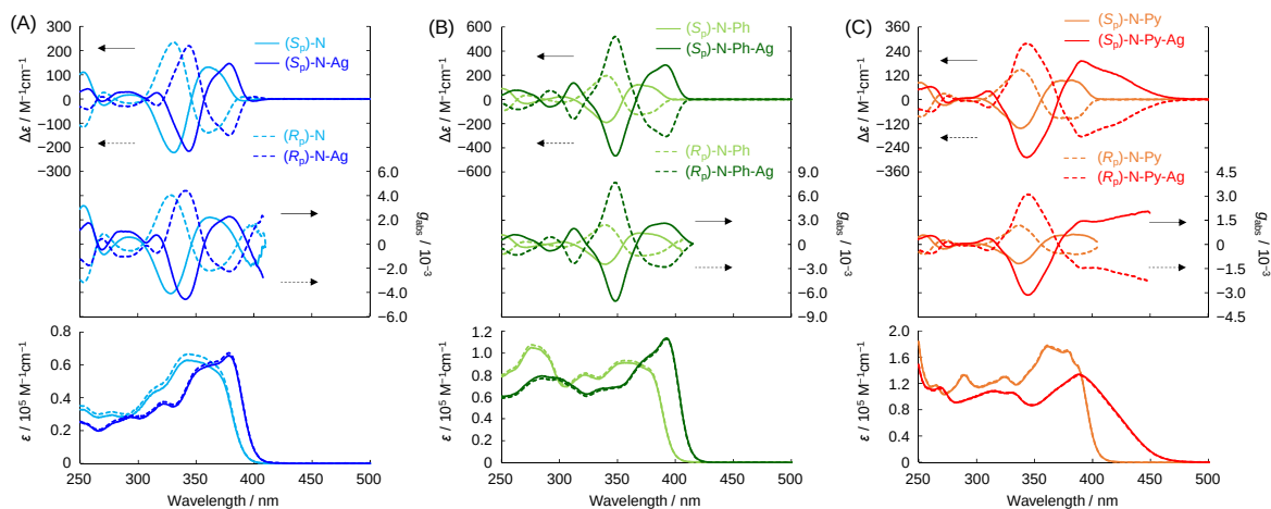
Figure 5. CD (top), g_{\text{abs}} (middle), and UV-vis absorption (bottom) spectra of (A) N and N-Ag in the dilute \text{CH}_2\text{Cl}_2 ( 1.0 \times 10^{-5} \text{ M} ), (B) N-Ph and N-Ph-Ag in the dilute \text{CH}_2\text{Cl}_2 ( 1.0 \times 10^{-5} \text{ M} ), (C) N-Py and N-Py-Ag in the dilute \text{CH}_2\text{Cl}_2 ( 5.0 \times 10^{-6} \text{ M} ).
