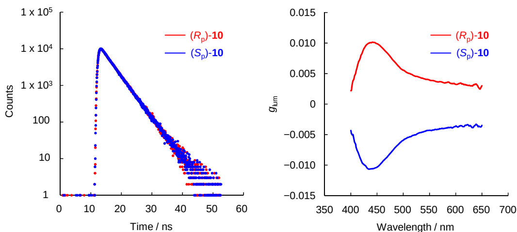
Figure 4. PL decay curves of ( R p )- and ( S p )- 10 in CHCl 3 ( 1.0 \times 10^{-5} M) at room temperature, excited at 375 nm LED laser.
