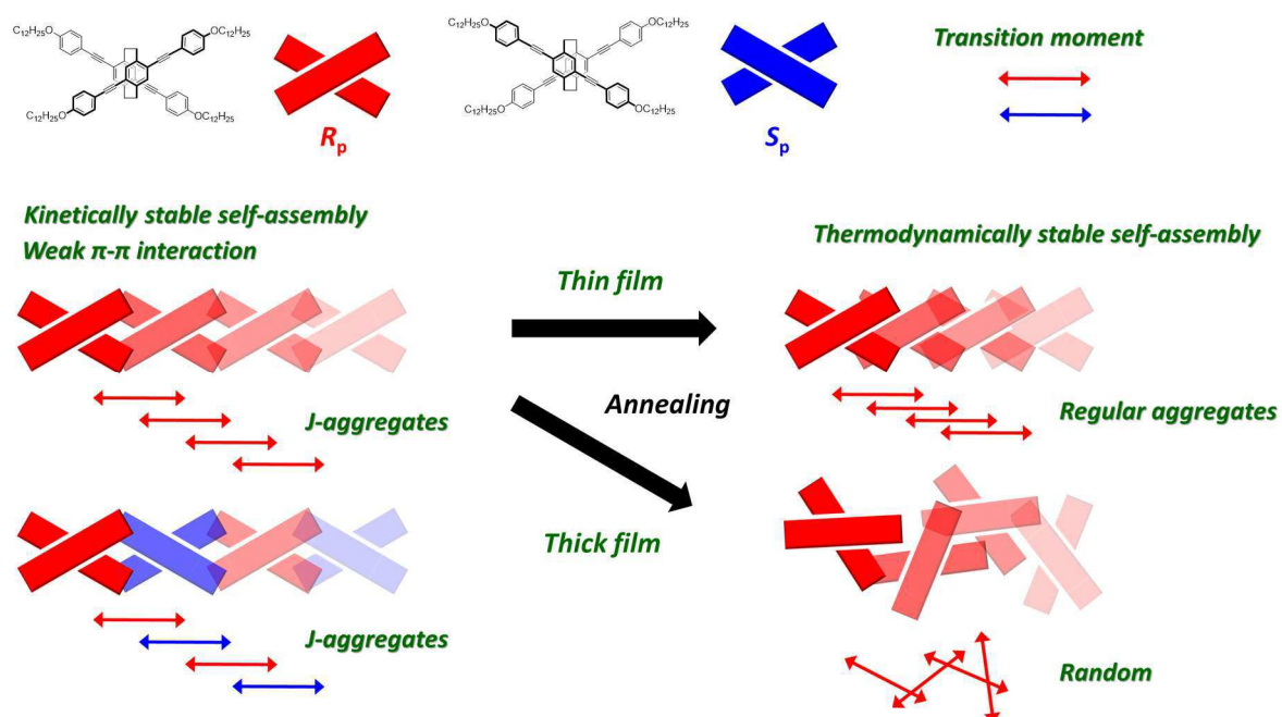
Figure 10. Proposal mechanism of Self-assembly of CP3 .
