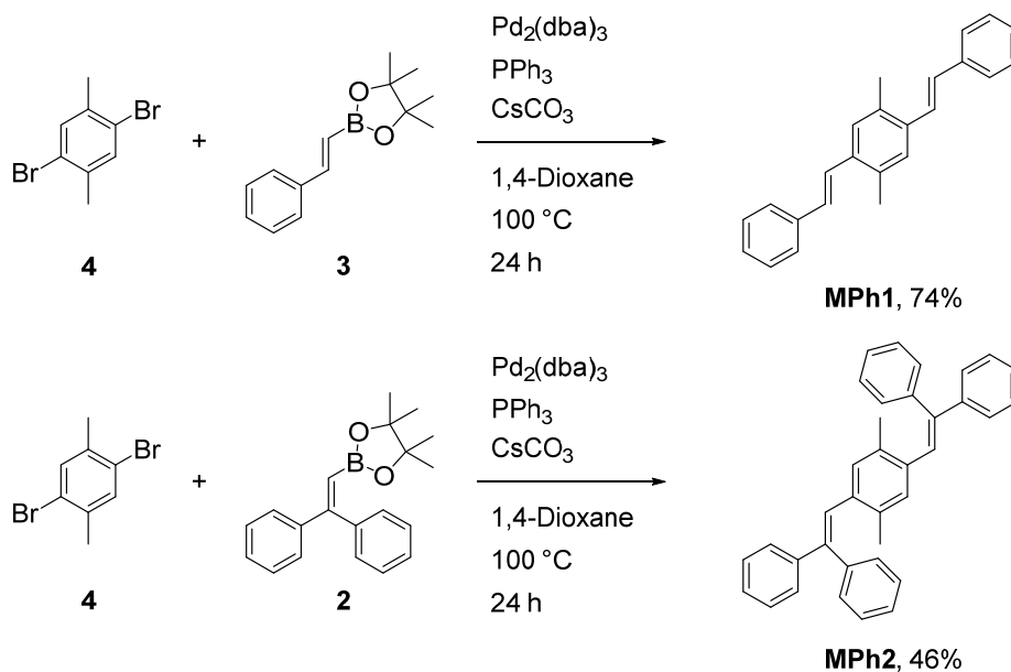
Scheme 3. Synthesis of model compounds MPh1 and MPh2
