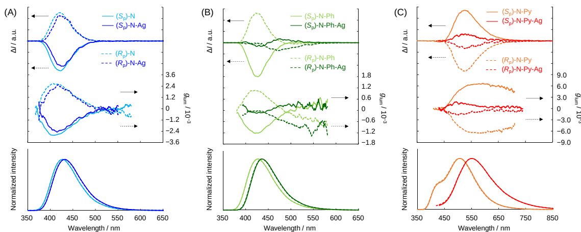
Figure 6. CPL (top), g_{\text{lum}} (middle), and PL (bottom) spectra of (A) N and N-Ag in the dilute \text{CH}_2\text{Cl}_2 ( 1.0 \times 10^{-5} \text{ M} ), (B) N-Ph and N-Ph-Ag in the dilute \text{CH}_2\text{Cl}_2 ( 1.0 \times 10^{-5} \text{ M} ), (C) N-Py and N-Py-Ag in the dilute \text{CH}_2\text{Cl}_2 ( 5.0 \times 10^{-6} \text{ M} ). Excitation wavelength was 300 nm (N, N-Ag, N-Ph, N-Ph-Ag and N-Py) and 350 nm (N-Py-Ag).
