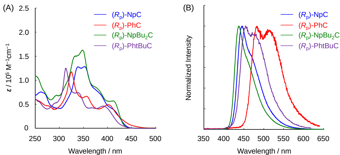
Figure 2. (A) UV-vis absorption spectra in the dilute \text{CHCl}_3 ( 1.0 \times 10^{-5} \text{ M} ) and (B) PL spectra in the dilute \text{CHCl}_3 ( 1.0 \times 10^{-6} \text{ M} ; excited at absorption maximum) of (R_p) -NpC, PhC, NpBu 2 C, and PhtBuC.
