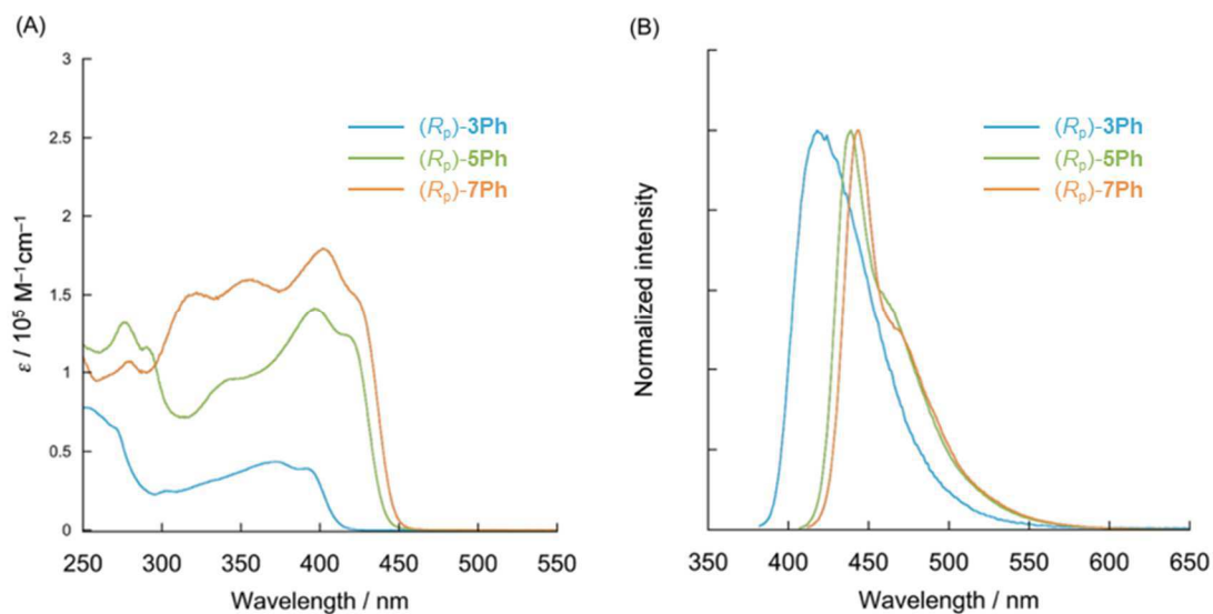
Figure 2. (A) UV-vis absorption spectra in the dilute \text{CHCl}_3 ( 1.0 \times 10^{-5} \text{ M} ) and (B) PL spectra in the dilute \text{CHCl}_3 ( 1.0 \times 10^{-5} \text{ M} ; excited at absorption maximum) of ( R p )- 3Ph , ( R p )- 5Ph , and ( R p )- 7Ph .
