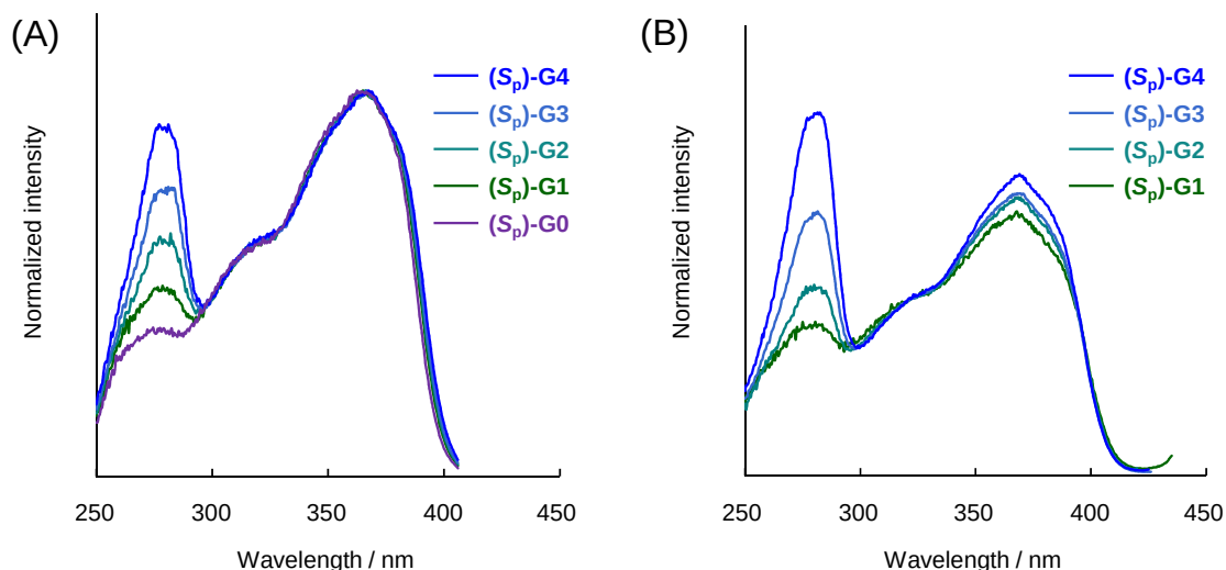
Figure 3. Excitation spectra of ( S p )- G0 , G1 , G2 , G3 , and G4 (A) in the dilute CHCl 3 ( 1.0 \times 10^{-5} M) and (B) in film prepared by a spin-coated method from CHCl 3 solution ( 1.0 \times 10^{-3} M). The spectra were normalized at each peak top in the range from 360 to 370 nm in the dilute CHCl 3 , and 325 nm in film.
