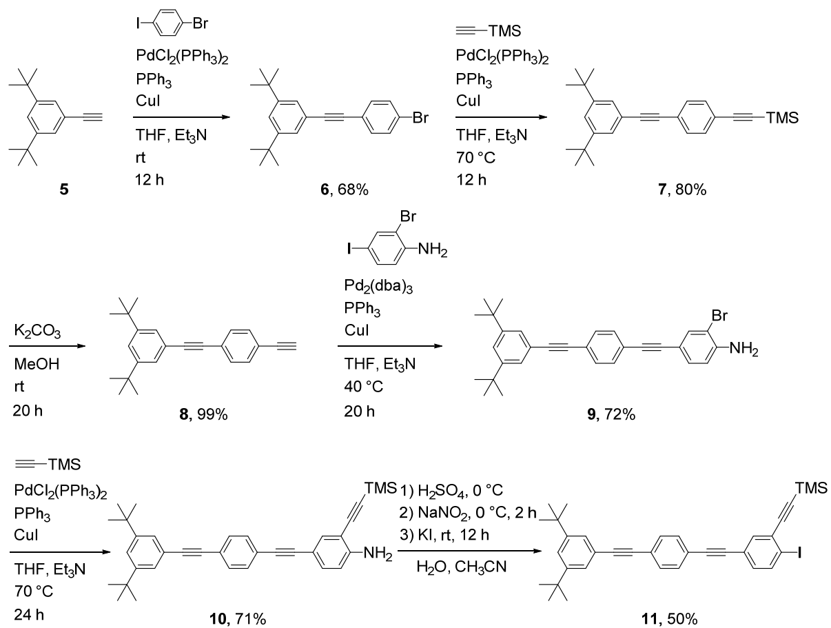
Scheme 2. Synthesis of compound 11 (arm unit for 7PhC )
