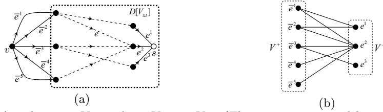
Fig. 7. (a) Arcs between V_{\leq t} and v \in V_{\leq t+1} - V_{\leq t} . (The arc e represented by a dotted line means that the tail of e is reachable to the head of e .) (b) G for v in (a).
