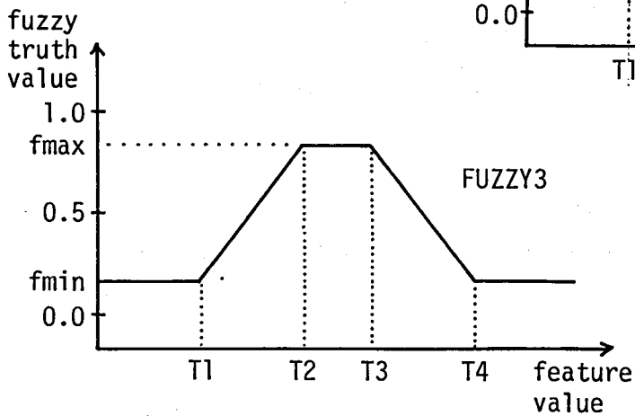
Figure 4-7. Three functions to define truth-value of fuzzy predicates from the feature value.
