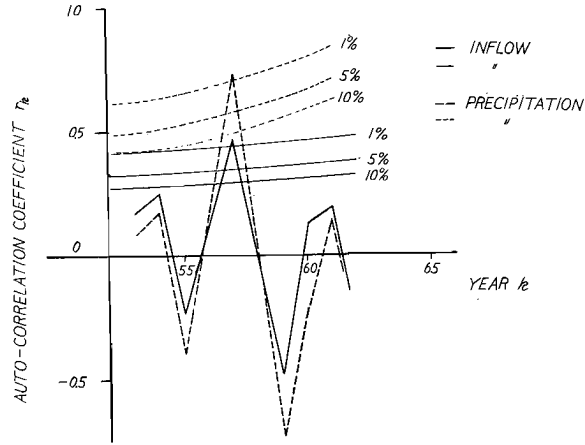
Fig. 3. Correlogram of summer inflow and precipitation for k=53 \sim 62 years.
