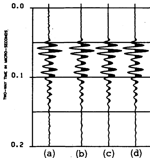
Fig. 5 Waves generated from ultrasonic transmitter
