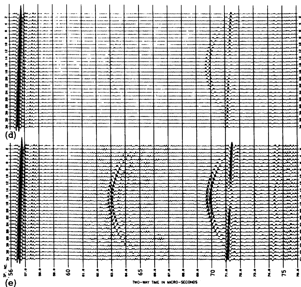
Fig. 7 Display of near trace section according to the processing sequence for wavelet processing
