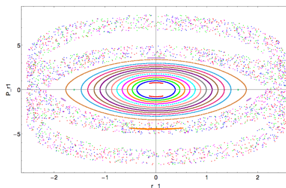
Figure 2. Improved Poincaré section with E = 10 .
