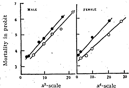
Fig. 1: Pre-narcotized influence on heat resistance compared by the regression line of probit-time in x^k scale.
