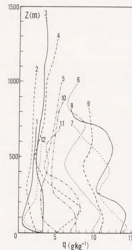
Fig. 4. Estimated monthly mean of the specific humidity profile estimated at the effective sunrise. The numbers on the profiles indicate the month.
