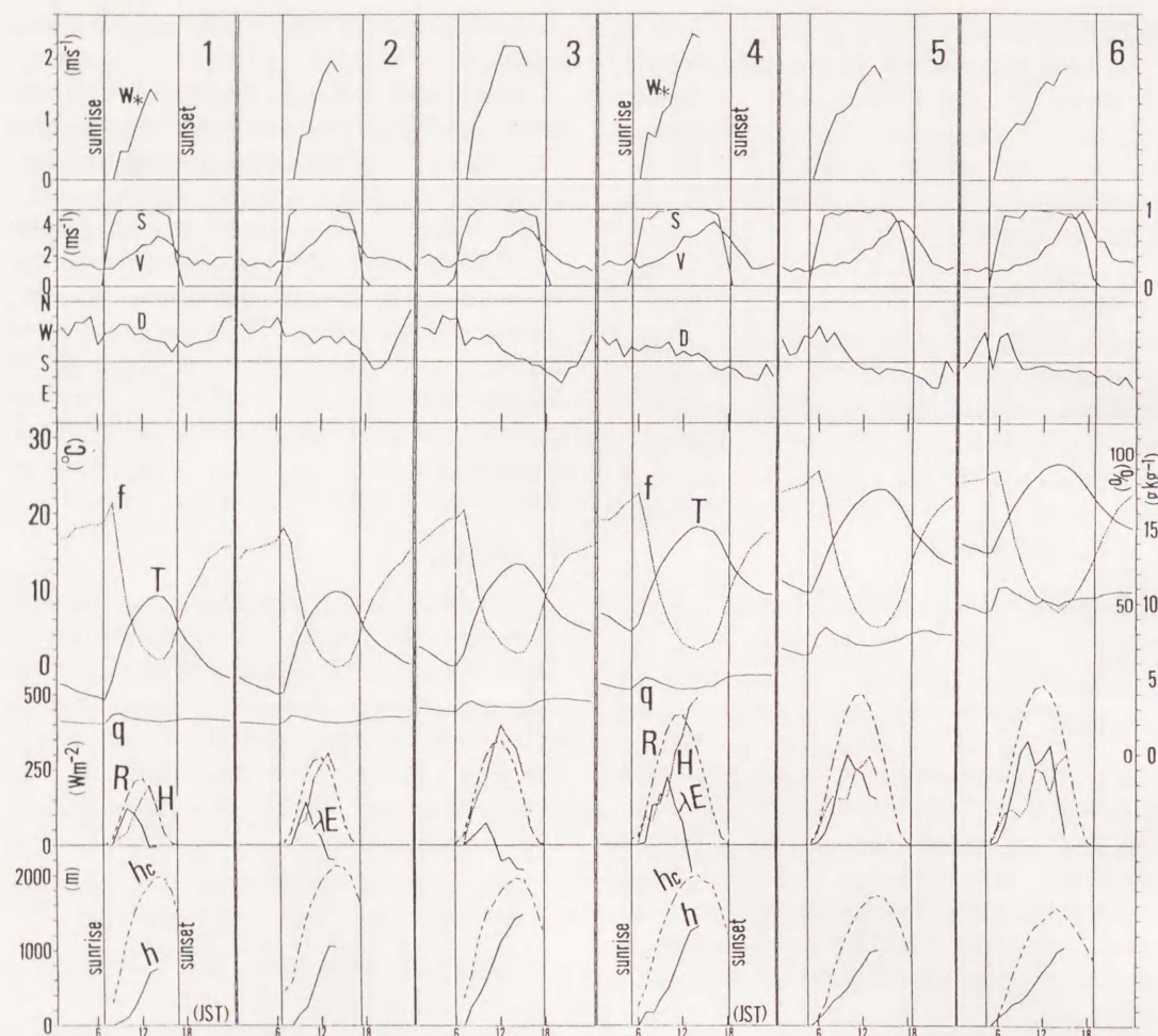
Fig. 3. Diurnal variation of the meteorological elements and the daytime trend of the mixed-layer characteristics for every month, averaged over five years from 1977 to 1981: V ( \text{ms}^{-1} ), wind speed (AMeDAS); D , wind direction (AMeDAS); S , duration of sunshine (AMeDAS); q ( \text{g kg}^{-1} ), specific humidity; f (%), relative humidity; T ( ^{\circ}\text{C} ), temperature; R ( \text{W m}^{-2} ), net radiation; H ( \text{W m}^{-2} ), surface sensible heat flux; \lambda E ( \text{W m}^{-2} ), surface latent heat flux; h (m), mixed layer height; h_c (m), lifting condensation level; W_* ( \text{ms}^{-1} ), convective velocity scale. The two vertical lines in each month show the sunrise and sunset.
