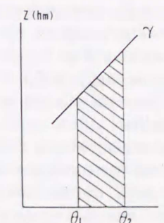
Fig. 1 Relationship between potential temperature in the mixed layer \theta(z) , mixed layer height h_m , and lapse rate \gamma . The lined area shows integrated surface sensible heat flux.
