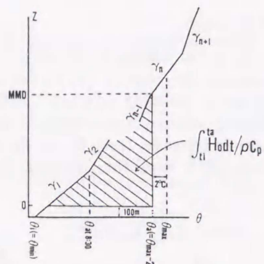
Fig. 2 Relationship between maximum mixing depth MMD, \gamma , and integrated surface heat flux \int_{t_i}^{t_a} H_0 dt . A time lag of radiosonde thermometer is assumed to be 100 m. The maximum potential temperature \theta_a in the mixed layer is assumed to be (\theta_{\max} - 2^\circ\text{C}) .
