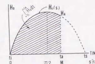
Fig. 15 Schematic figure representing the manner how to estimate the hourly variation of the sensible heat flux H_0 from the integrated value ( \int_{t_i}^{t_a} H_0 dt ). H_a is heat flux at time t_a .
