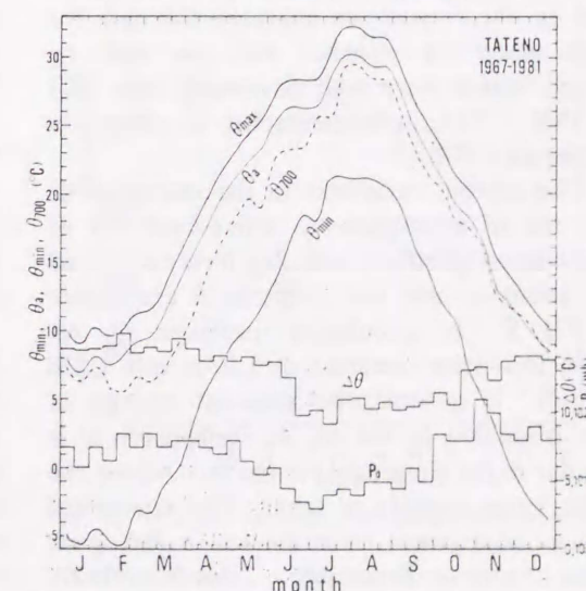
Fig. 8 Annual variations of \theta_{\max} , \theta_a , \theta_{\min} , potential temperature at a height of 700 m, \theta_{700} , and surface pressure P_0 for days when the mixed layers are developed.
