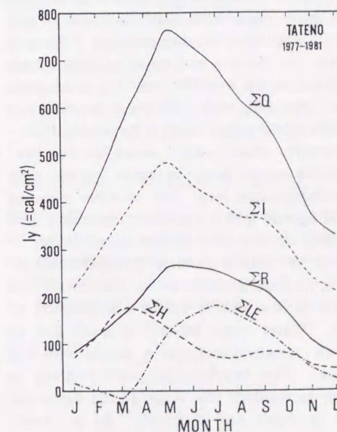
Fig. 12 Annual variations of energy balance components integrated from t_i to t_a at Tateno: \Sigma Q , insolation at the top of atmosphere; \Sigma I , downward flux of short-wave radiation; \Sigma R , net radiation; \Sigma H (= \int_{t_i}^{t_a} H_0 dt) , surface sensible heat flux; \Sigma LE (= \Sigma R - \Sigma H) , surface latent heat flux.
