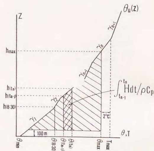
Fig. 1. The relationship between potential temperature in the mixed-layer \theta , mixed-layer height h , and lapse rate \gamma . t_n denotes the n hrs from the effective sunrise t_I . The hatched area shows the surface heat flux supplied into the mixed layer in the time interval between t_{n-1} and t_n . \theta_{\min} is the temperature at t_I . (8:30) means the time when the rawinsonde is launched. T_{\max} and \theta_{\max} are daily maximum values of low-level temperature, and potential temperature throughout the mixed layer. h_{\max} is the maximum mixing depth.
