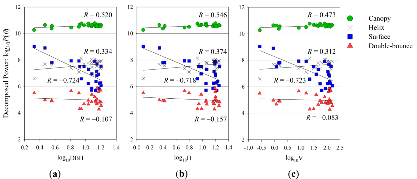
Figure 6. (a–c) Same as in Figure 5(a–c), except the decomposition powers are calculated from the rotated covariance matrix of \log_{10}P_{s(\theta)} , \log_{10}P_{d(\theta)} , \log_{10}P_{c(\theta)} and \log_{10}P_{h(\theta)} on the y-axis.
