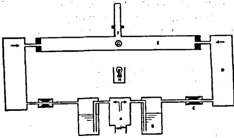
Fig 2. Diagram of an olfactometer
