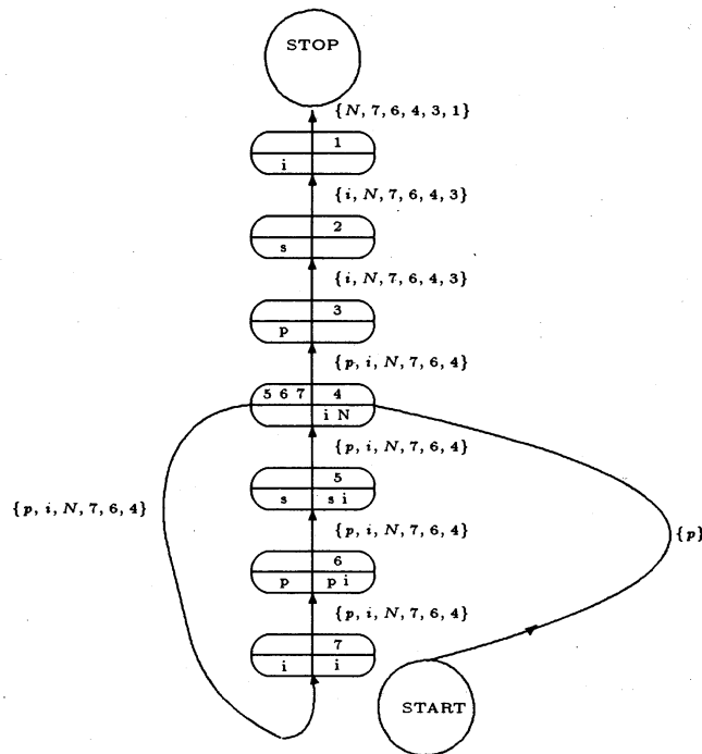
Figure 6: Final Network State
