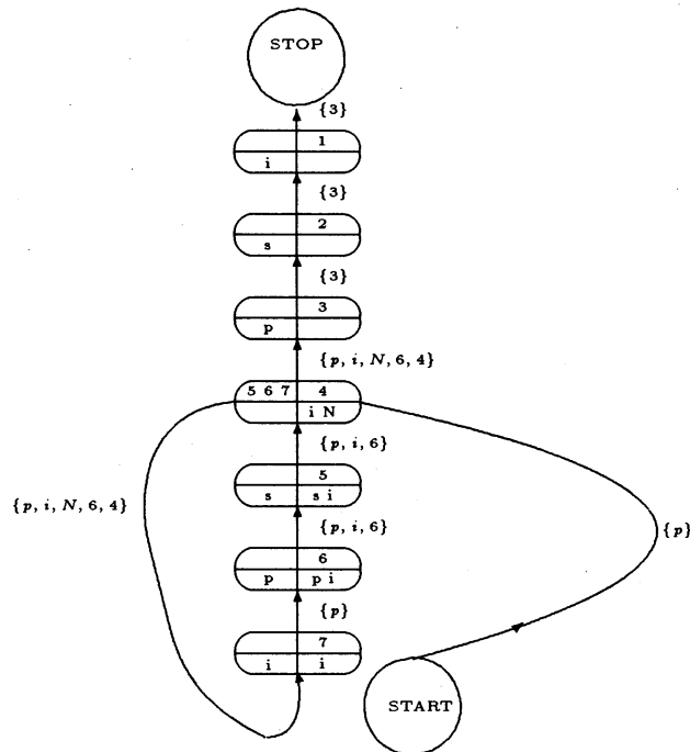
Figure 5: An intermediate Network State
