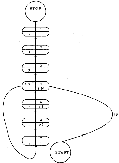
Figure 3: Initial Network State
