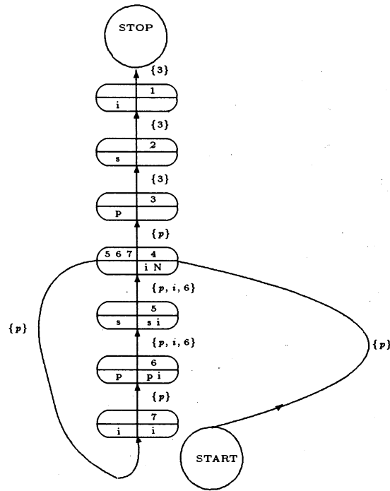
Figure 4: An intermediate Network State
