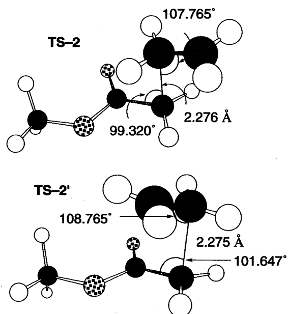
Figure 2. Transition Structures of the Radical Addition Step (Step 2 and Step 2')
