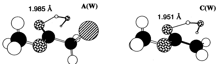
Figure 6. Optimized Structures of A(W) and C(W)
