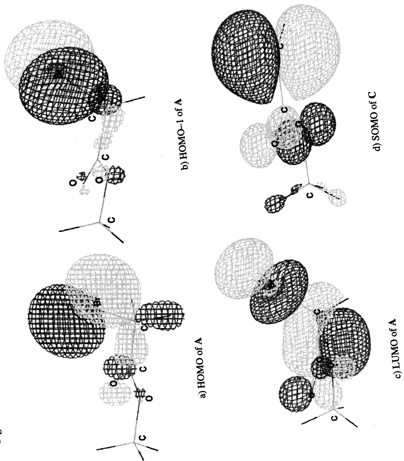
Figure 5. Molecular Orbitals of A and C
