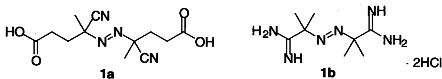
Figure 1. Water-soluble radical initiators
