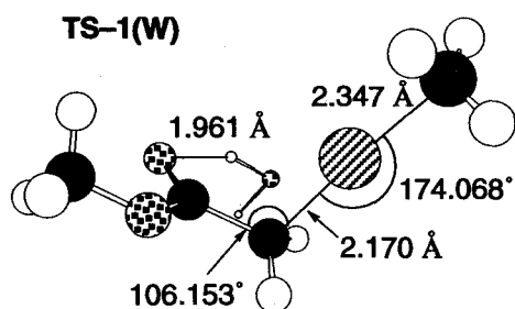
Figure 3. Transition Structure of Step 1 with Explicit Water
