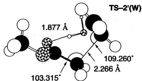
Figure 4. Transition Structures of Step 2 and 2' with Explicit Water
