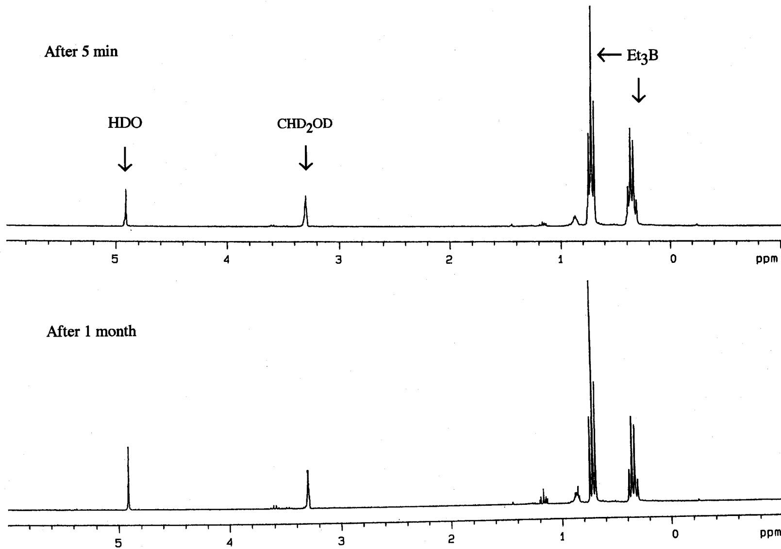
Fig. 1 ^1\text{H} NMR Spectra of Triethylborane in Methanol- d_4 (0.25 M)
