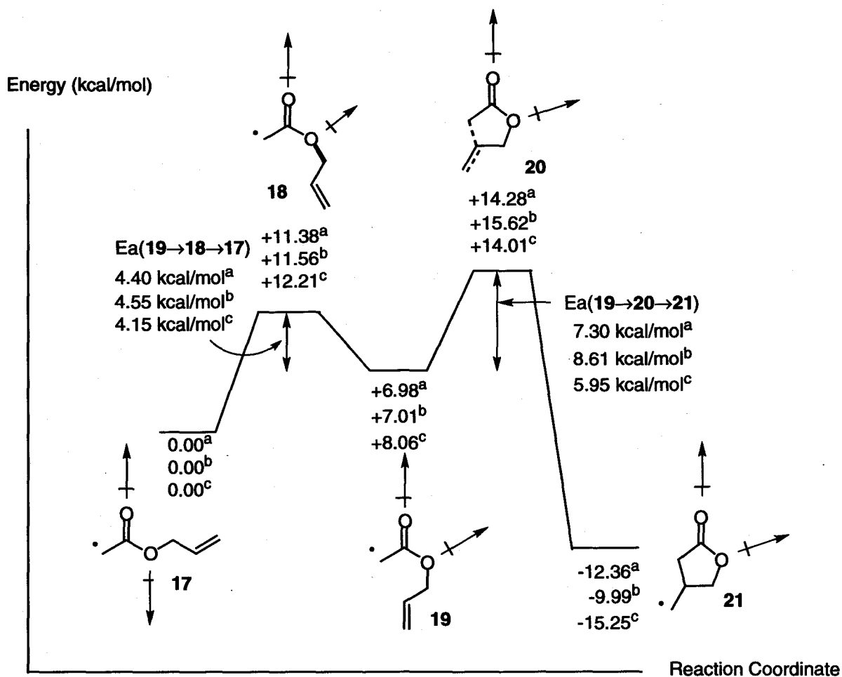
Scheme 10. Calculated energy profile for the transformation of Z-(allyloxycarbonyl)methyl radical into its cyclized form in vacuum. An arrow with a crossed end symbolizes a dipole moment that makes a large contribution to the net dipole moment of a molecule.
