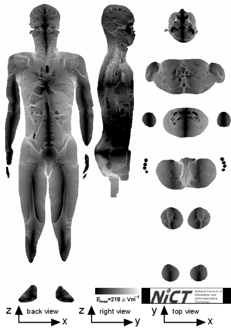
Figure 3. Electric field distributions and layer-maximum, layer-averaged, tissue-maximum, and tissue-averaged electric field strength ( \mu\text{Vm}^{-1} ) induced by 1 \mu\text{T} (peak), 50Hz, uniform B_j (back-to-front) magnetic fields
