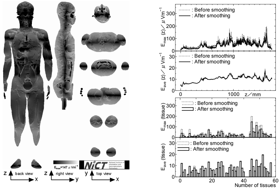
Figure 2. Electric field distributions and layer-maximum, layer-averaged, tissue-maximum, and tissue-averaged electric field strength ( \mu\text{Vm}^{-1} ) induced by 1 \mu\text{T} (peak), 50Hz, uniform Bi (left-to-right) magnetic fields
