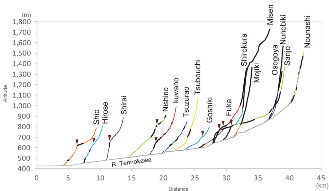
Fig. 5 Channel profiles of major tributaries. Thick black line shows the reaches with resistant rocks (Fig. 4).
