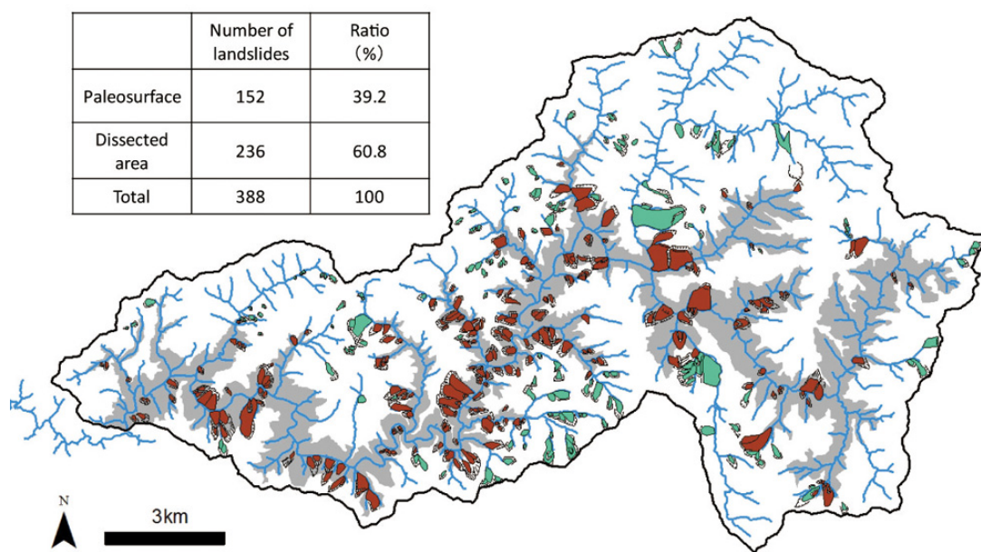
Fig. 6 Distribution of landslide bodies (using Landslide Distribution Maps by National Research Institute for Earth Science and Disaster Prevention). Green: landslides within the paleosurface. Brown: landslides on the dissected areas totally or partly.
