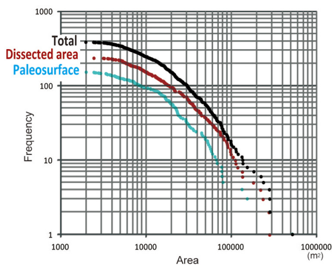
Fig. 7 Cumulative landslide frequency and the landslide size.
