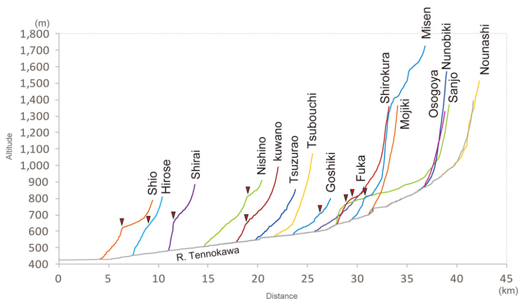
Fig. 3 Channel profiles of sixteen major tributaries and manually identified knickpoints.
