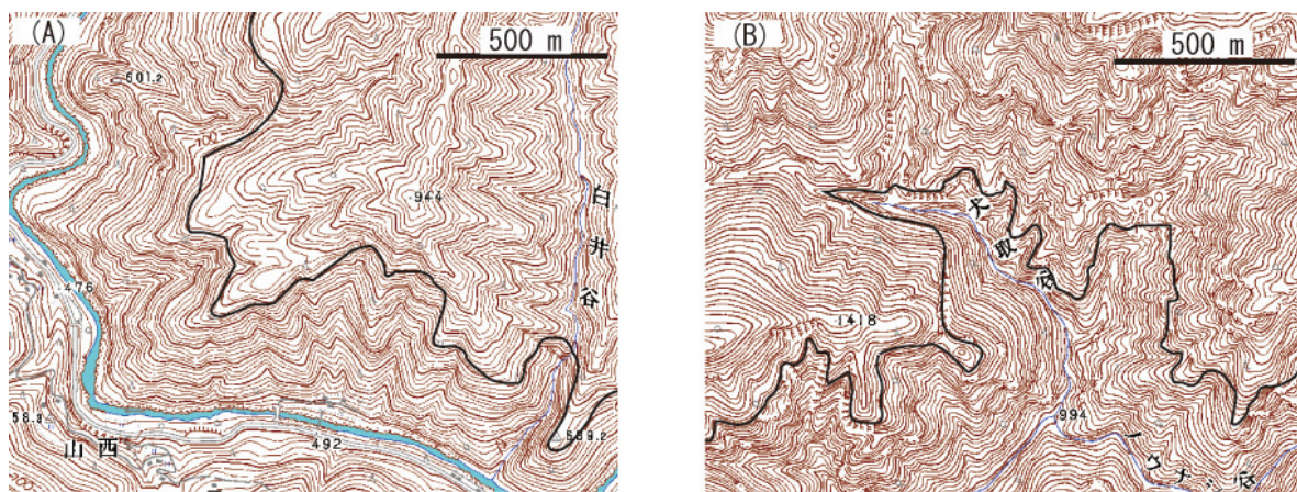
Fig.10 Examples of topographic maps in the study area, showing the slope breaks L1. Contour interval is 10 m. The base map used is “Minamihiura” (A) and “Misen” (B) with a scale of 1:25,000 by the Geospatial Information Authority of Japan. Black line shows upper slope break L1. (A) A clearly defined slope break line in the west part of study area. (B) A slope break line in the east part of study area. The contrast in slopes is not so strong as in the west part of study area.
